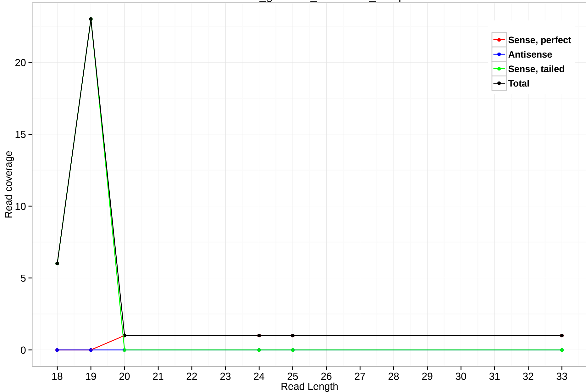
rheMac3_genscan_chr1.1734_14.3p
