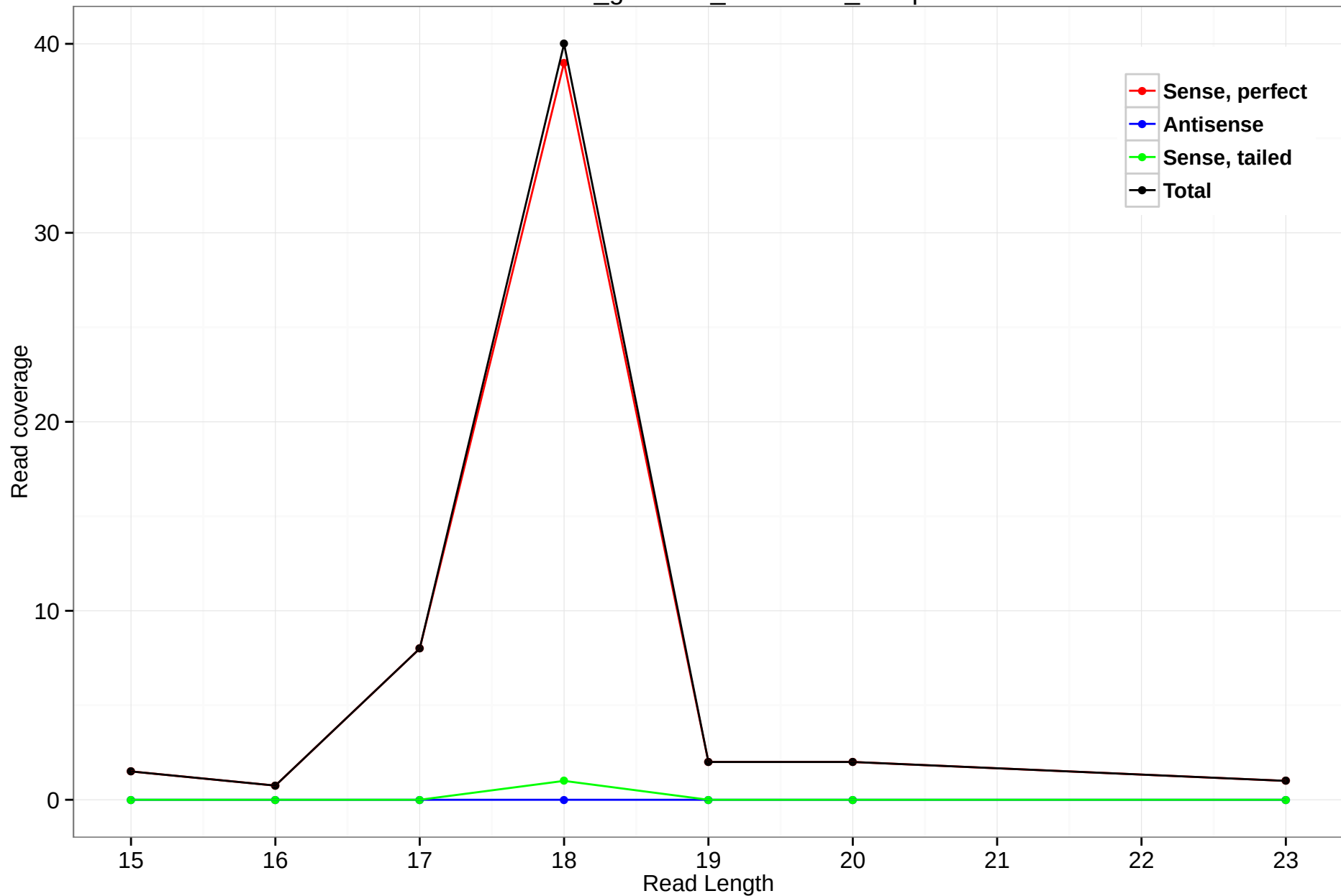
rheMac3_genscan_chr1.1731_19.5p
