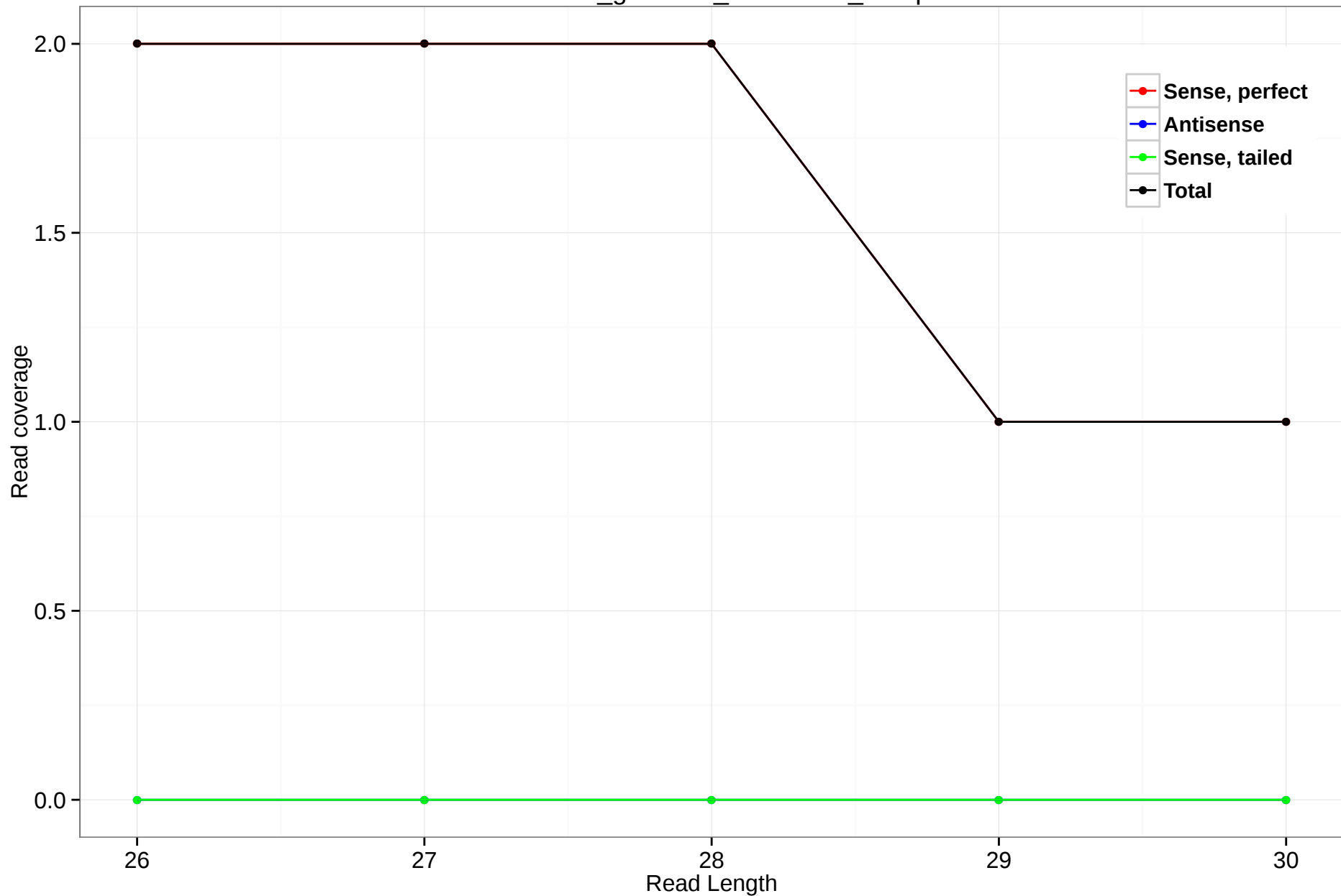
rheMac3_genscan_chr1.1731_18.5p
