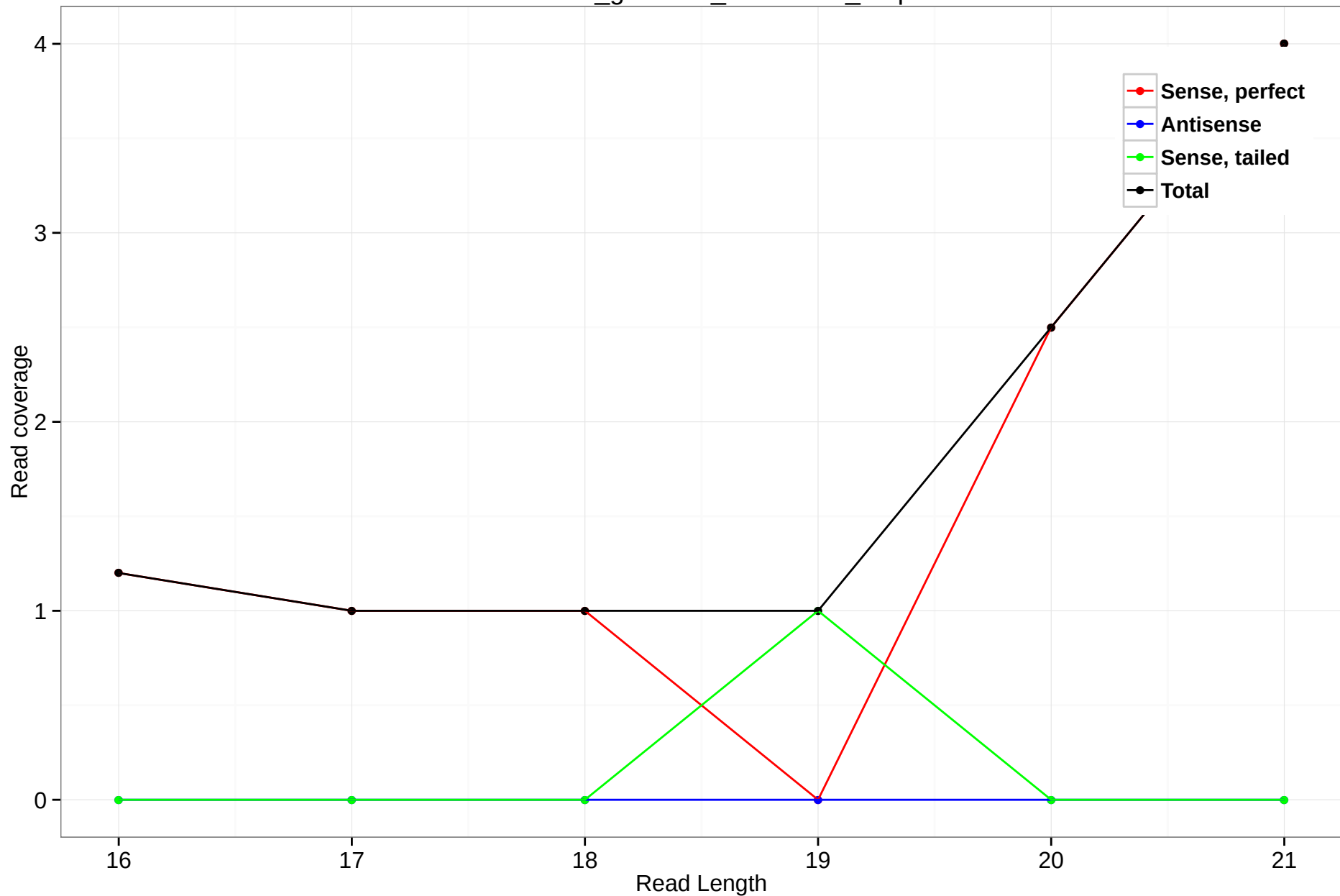
rheMac3_genscan_chr1.1712_0.3p
