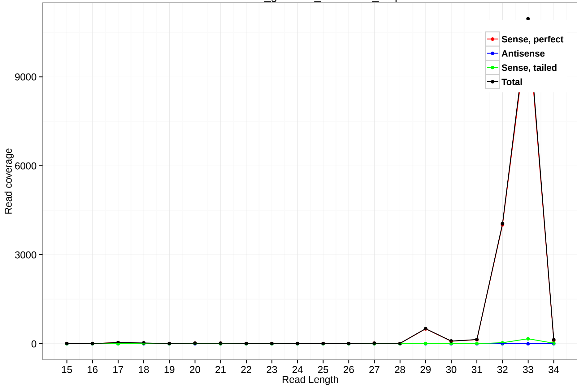
rheMac3_genscan_chr1.1704_9.5p
