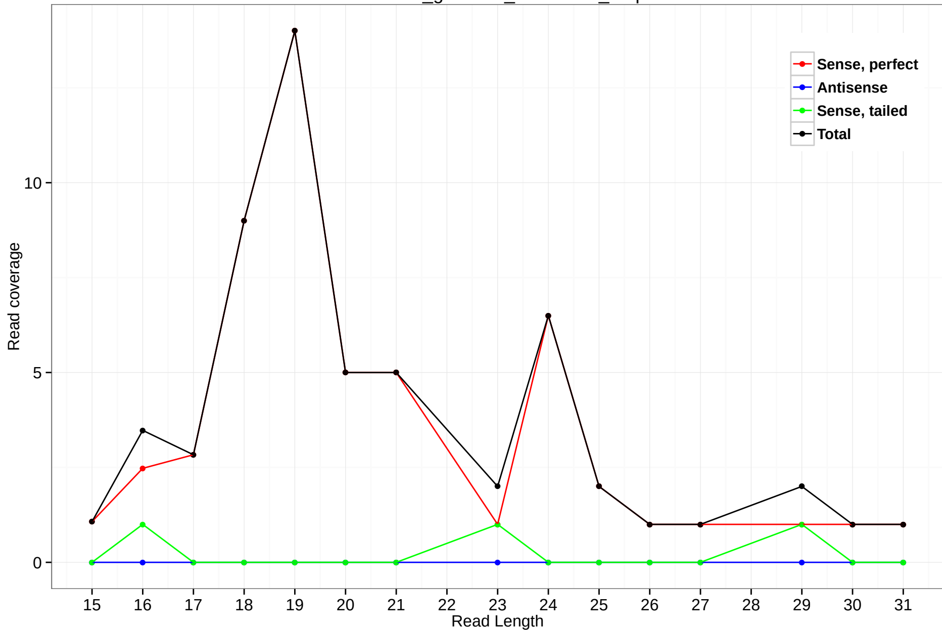
rheMac3_genscan_chr1.1656_0.3p
