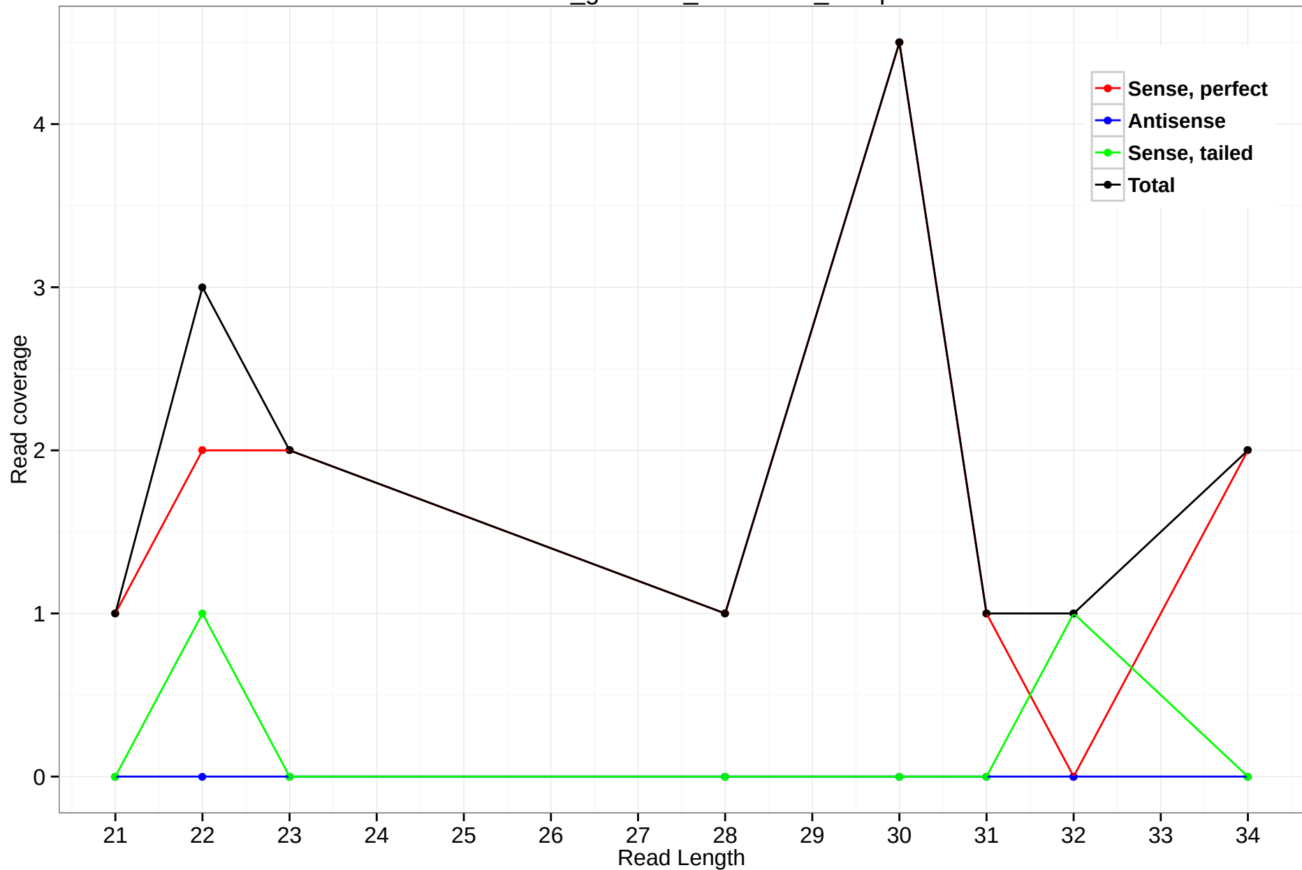
rheMac3_genscan_chr1.1625_13.3p
