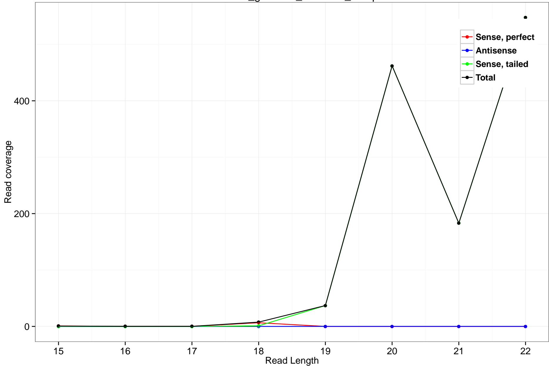
rheMac3_genscan_chr1.144_13.5p
