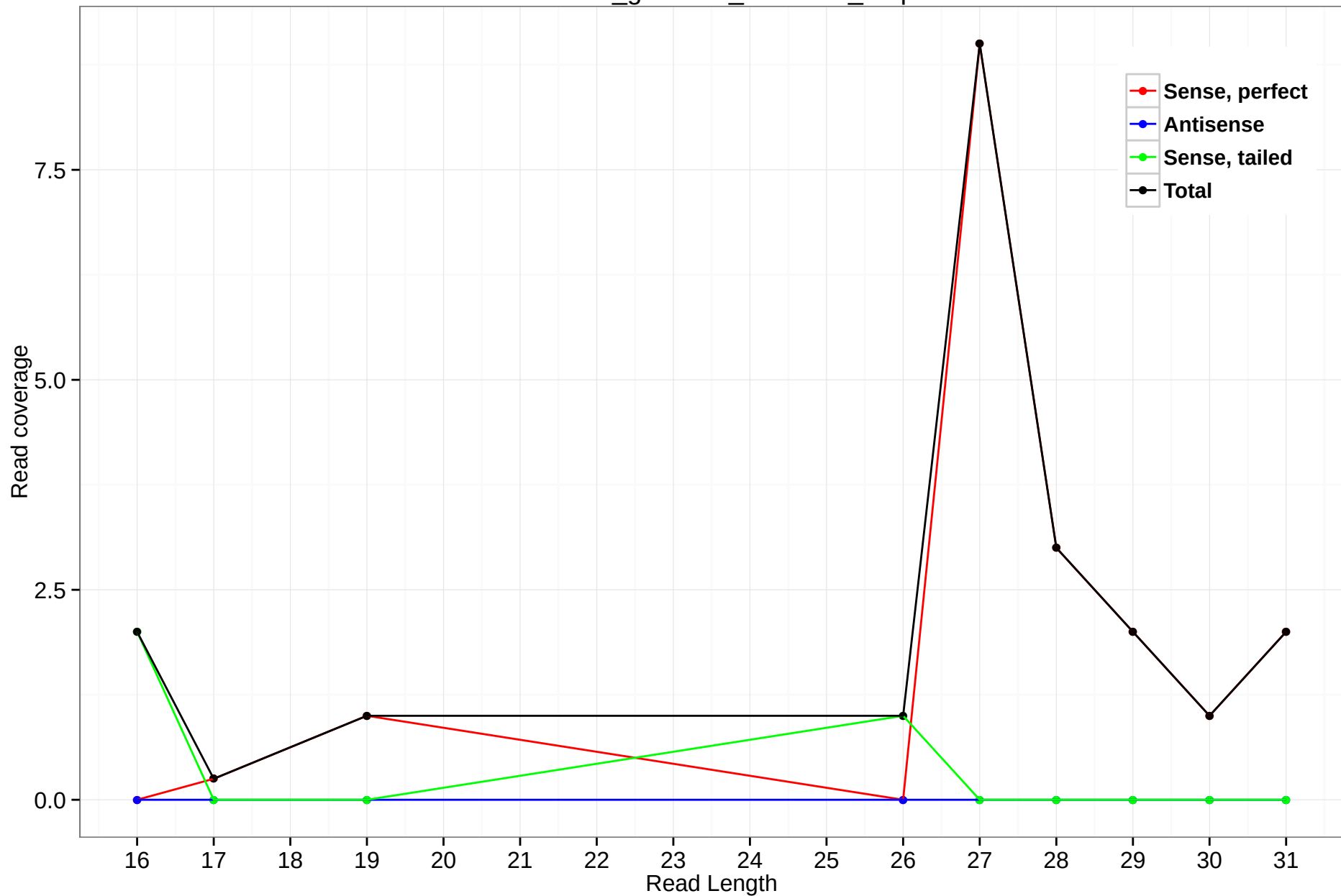
rheMac3_genscan_chr1.142_2.3p
