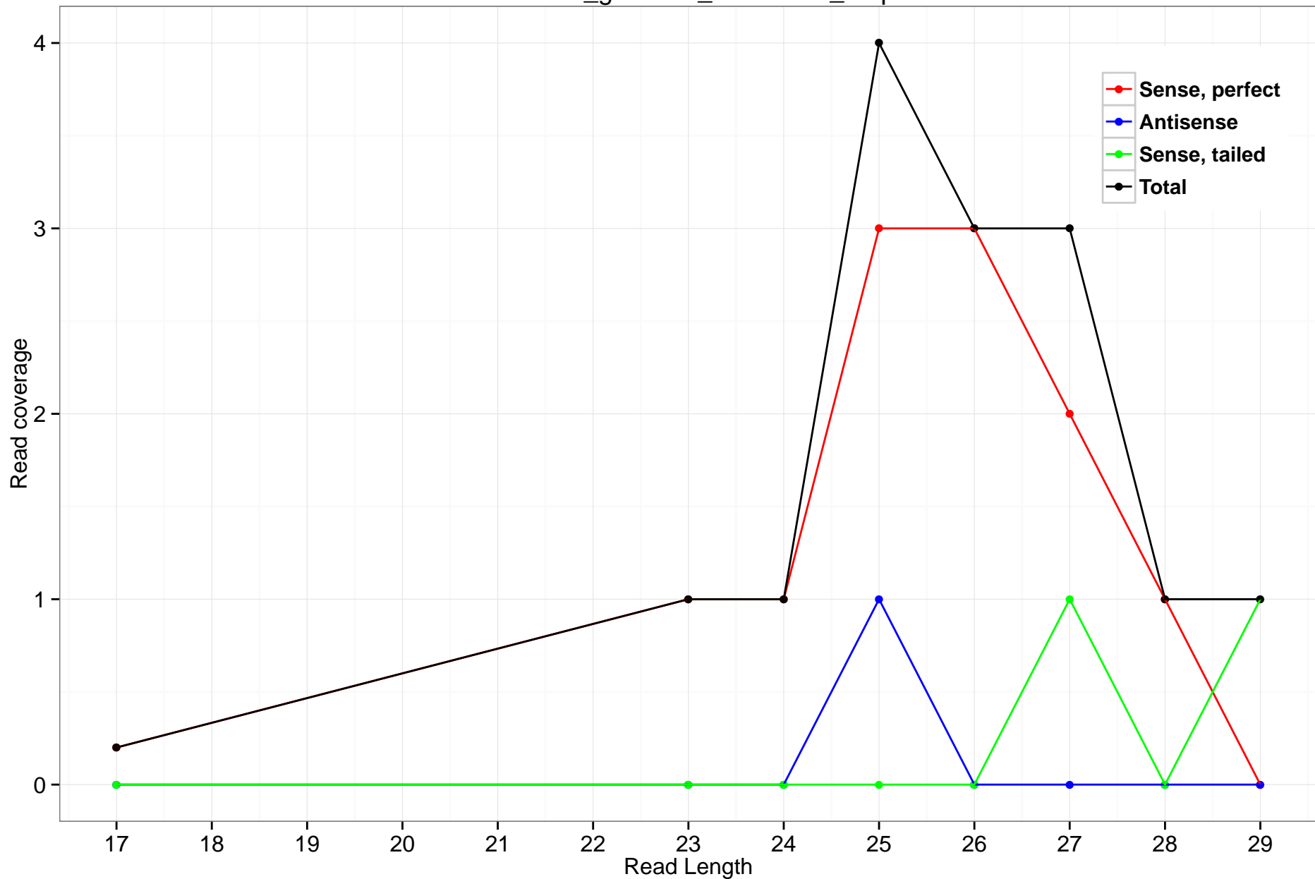
rheMac3_genscan_chr1.1384_5.5p
