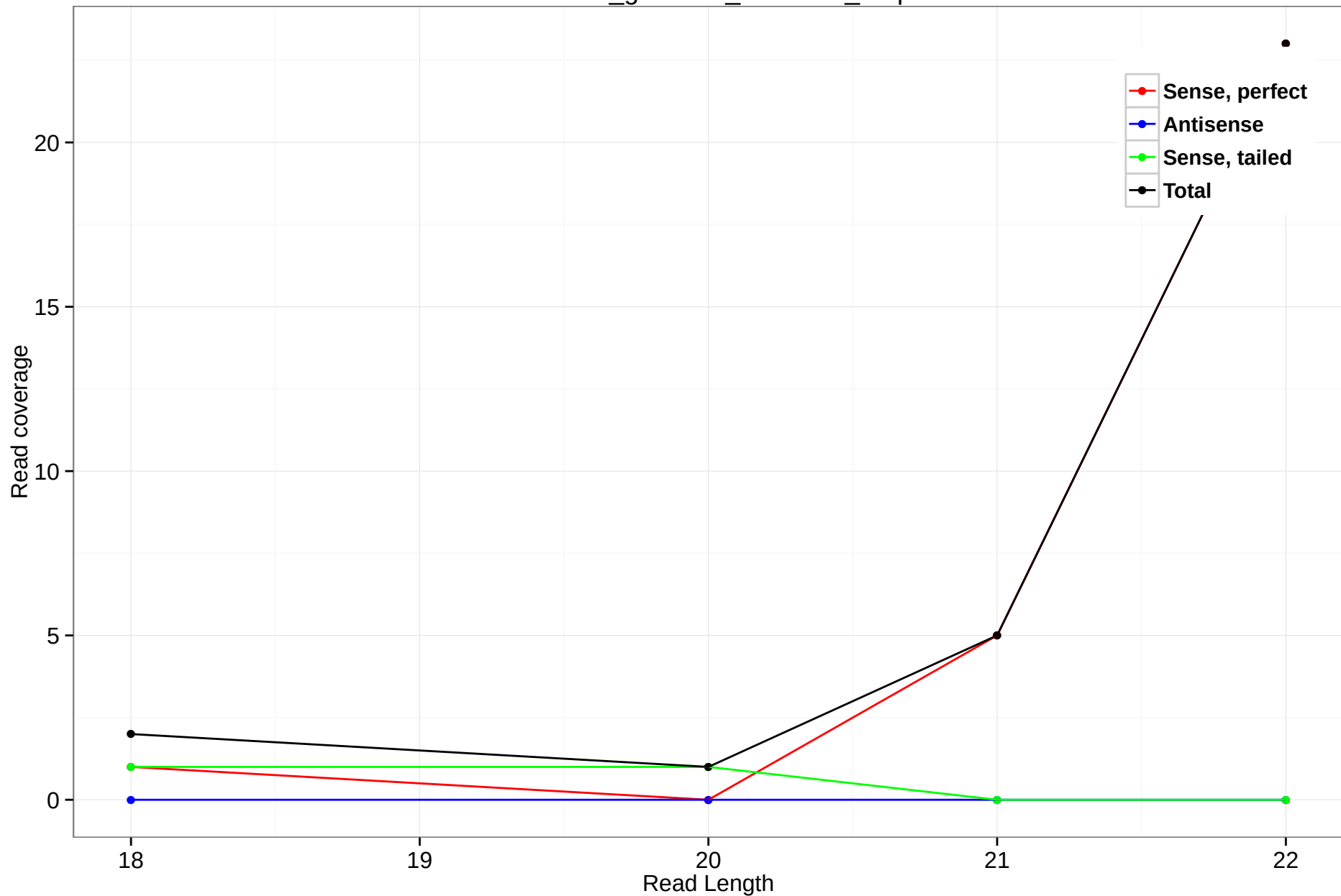
rheMac3_genscan_chr1.135_4.3p
