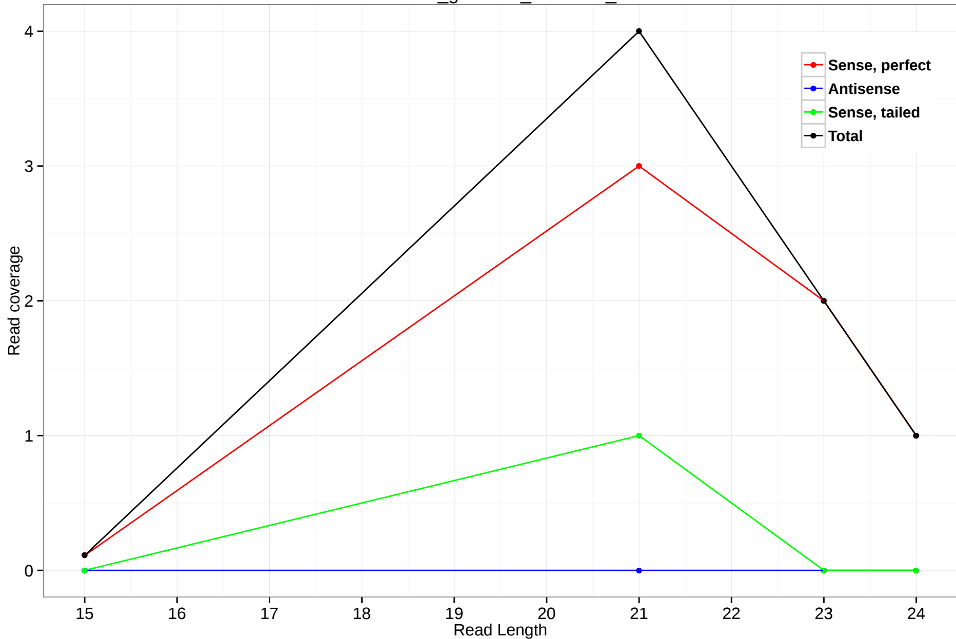
rheMac3_genscan_chr1.135_16
