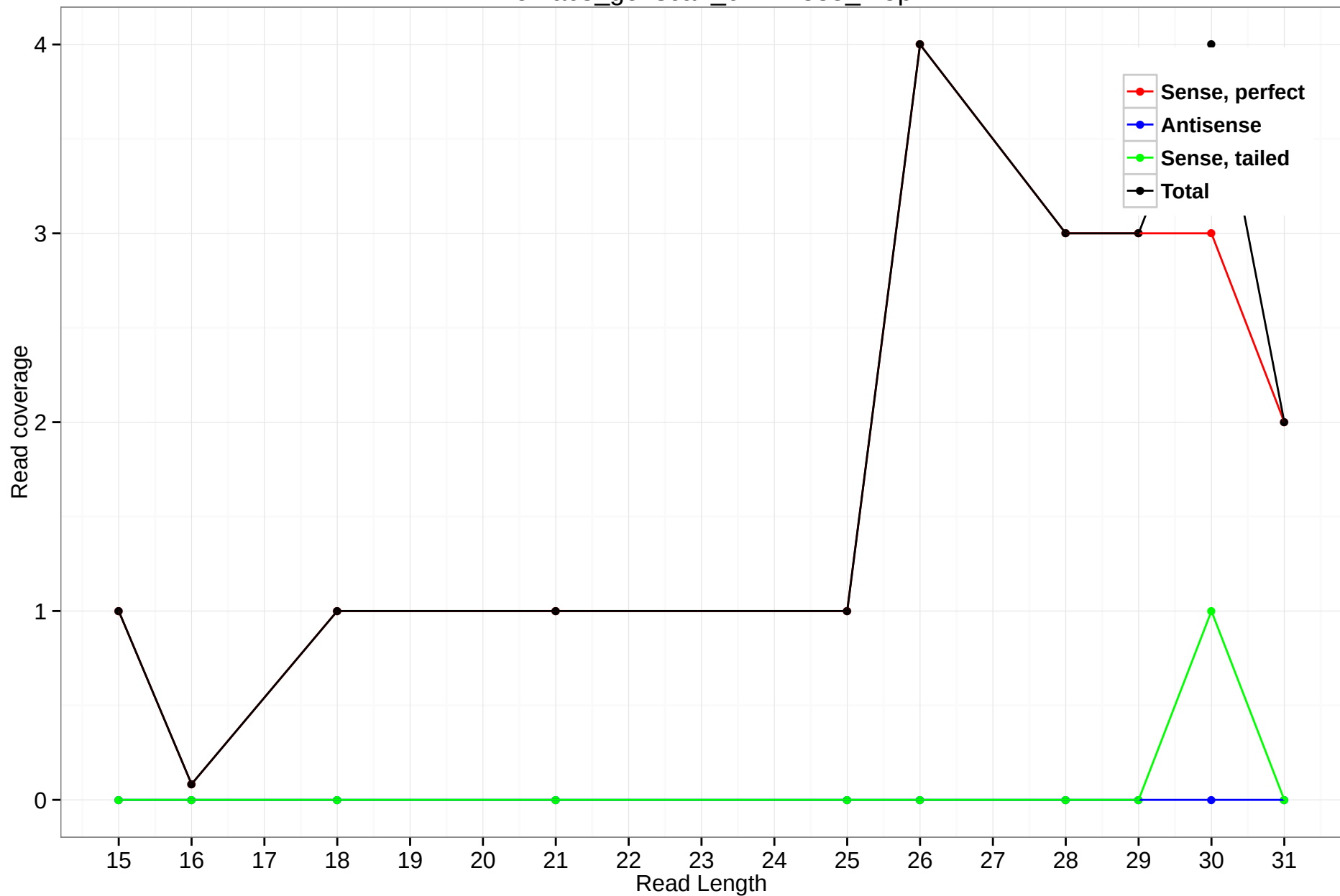
rheMac3_genscan_chr1.1335_1.5p
