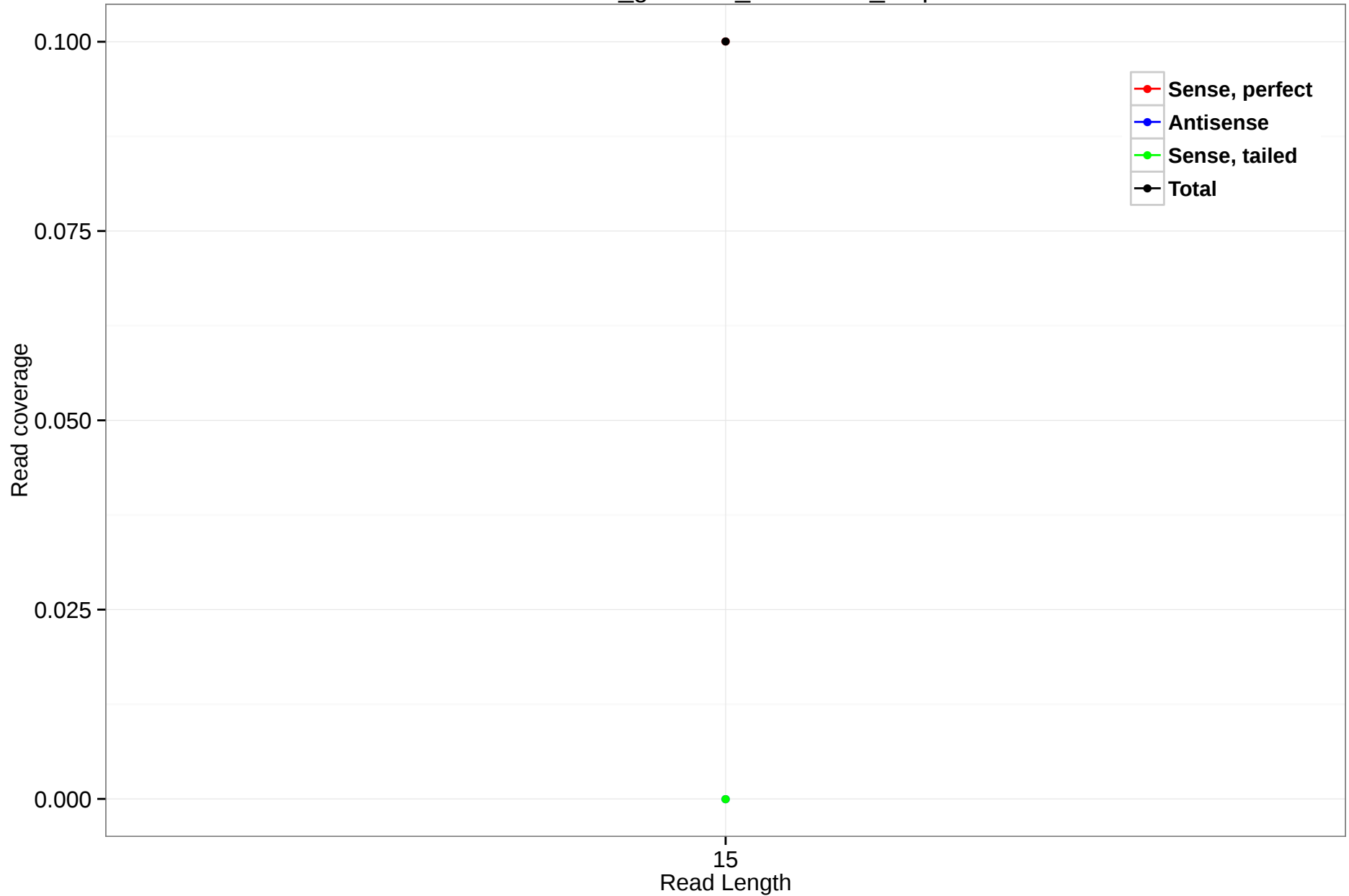
rheMac3_genscan_chr1.1332_0.3p
