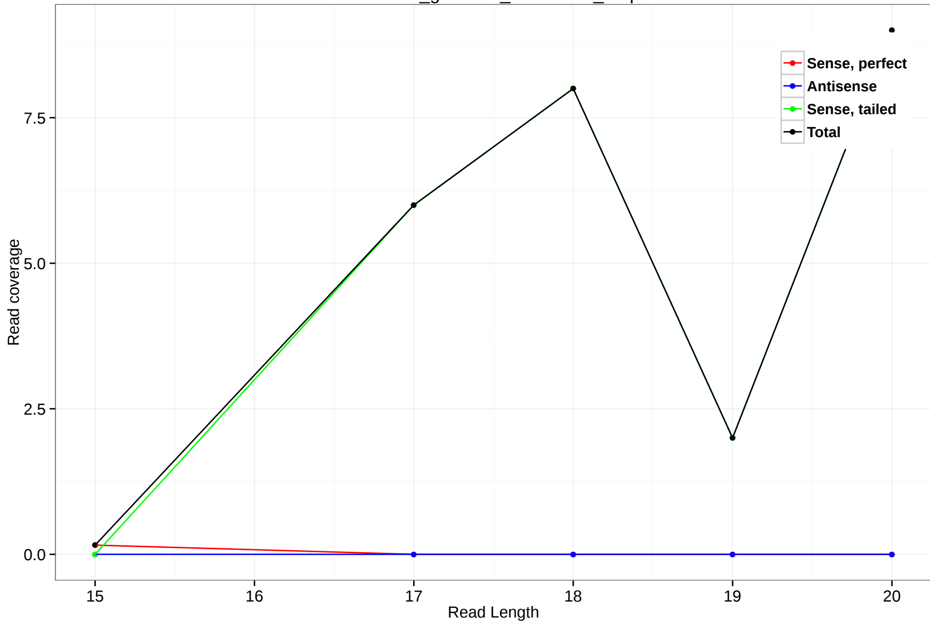
rheMac3_genscan_chr1.1263_5.5p
