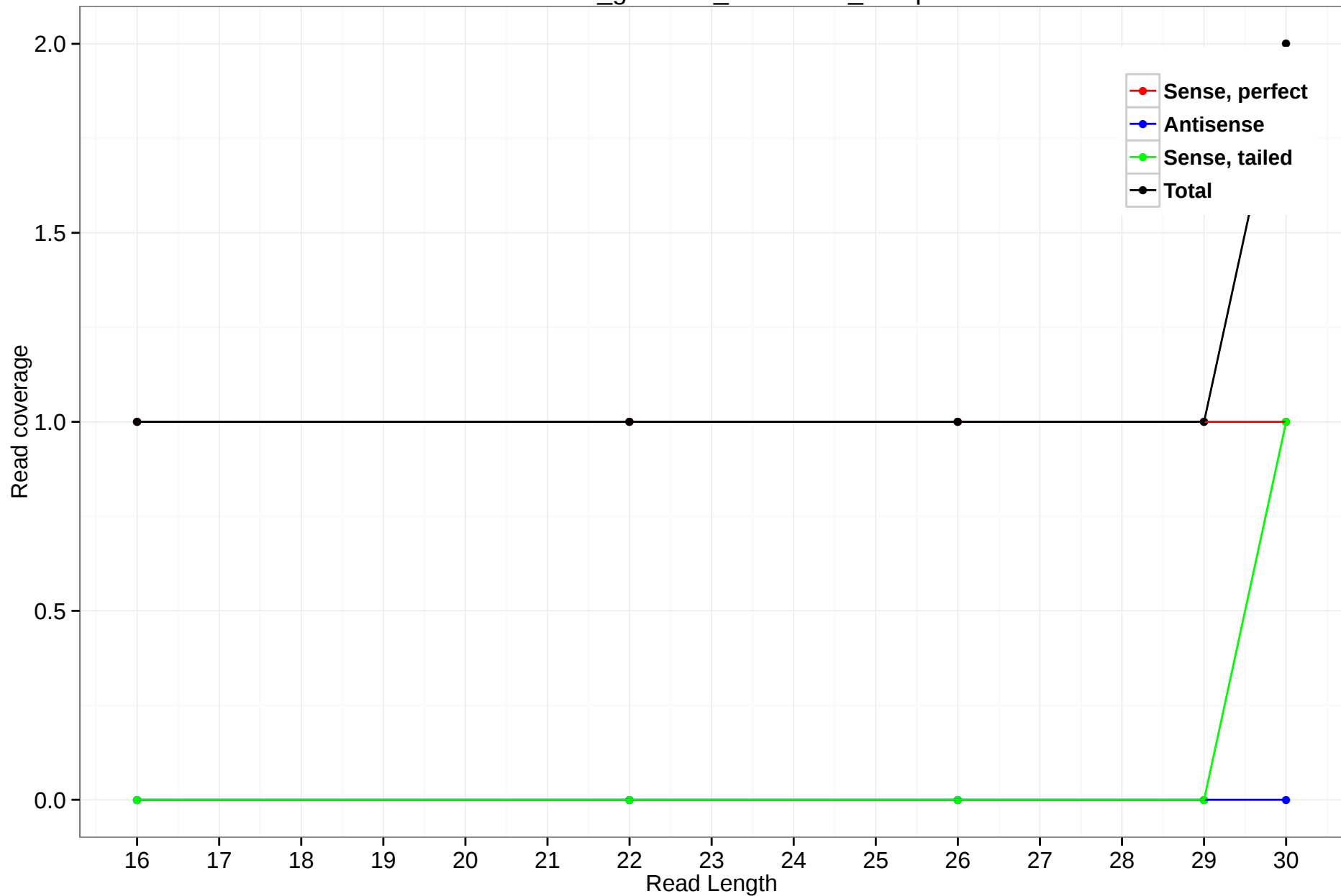
rheMac3_genscan_chr1.1218_12.3p
