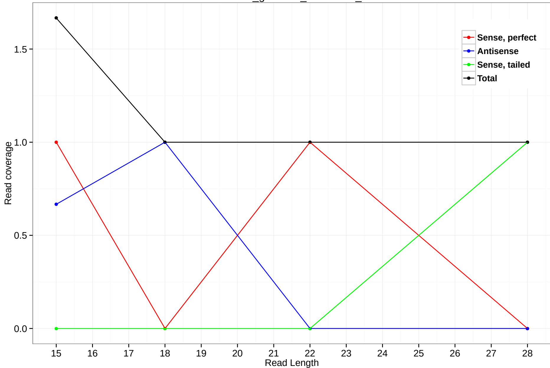
rheMac3_genscan_chr1.1182_12
