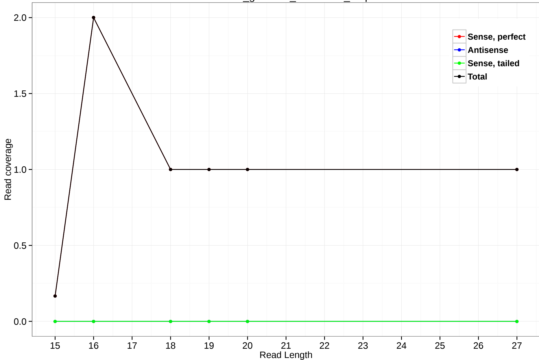
rheMac3_genscan_chr1.1154_9.3p
