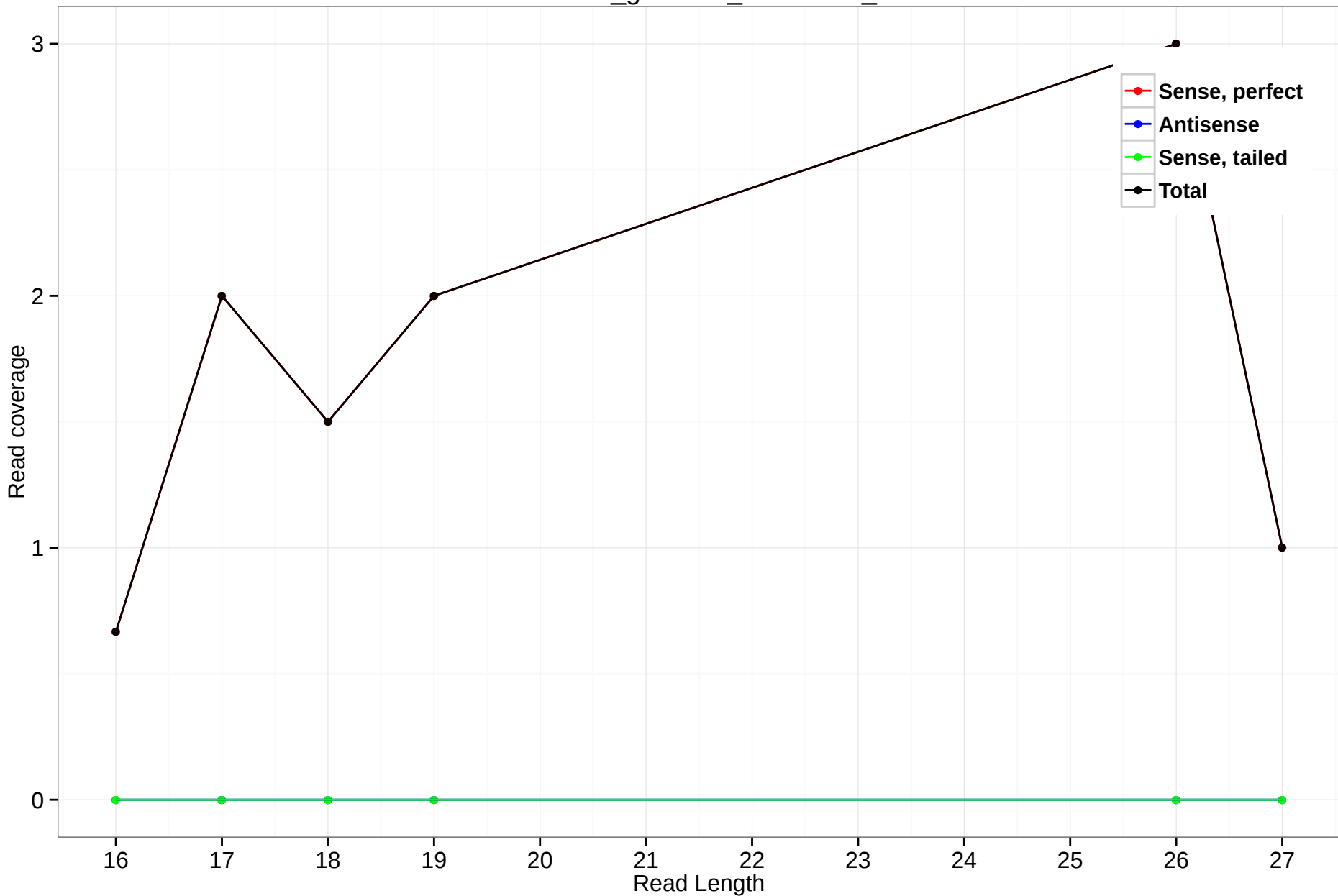
rheMac3_genscan_chr1.1150_0
