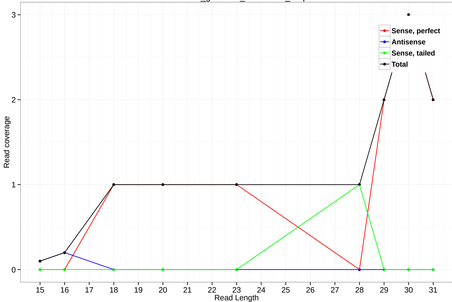
rheMac3_genscan_chr1.1144_3.5p
