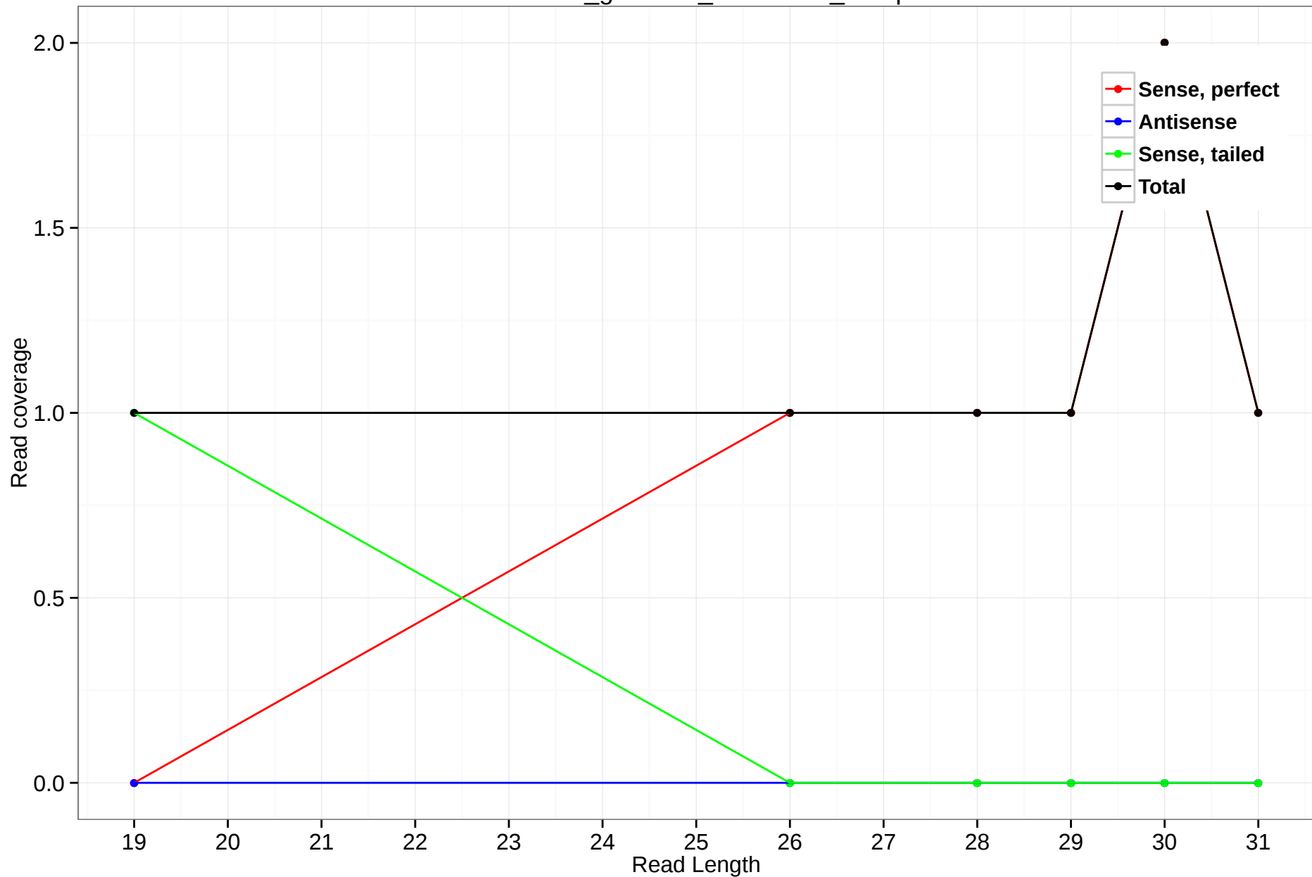
rheMac3_genscan_chr1.1144_18.5p
