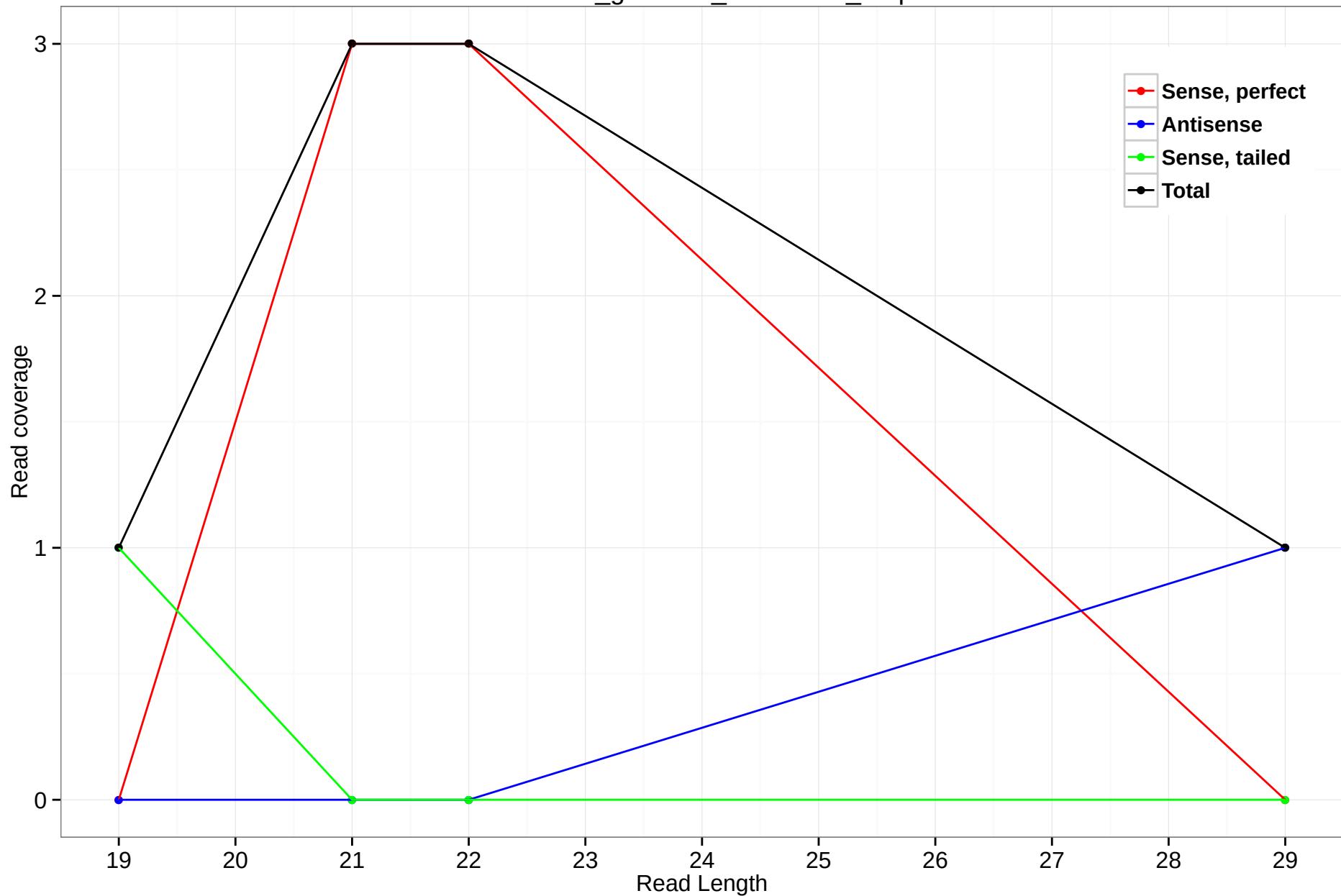
rheMac3_genscan_chr1.1110_1.3p
