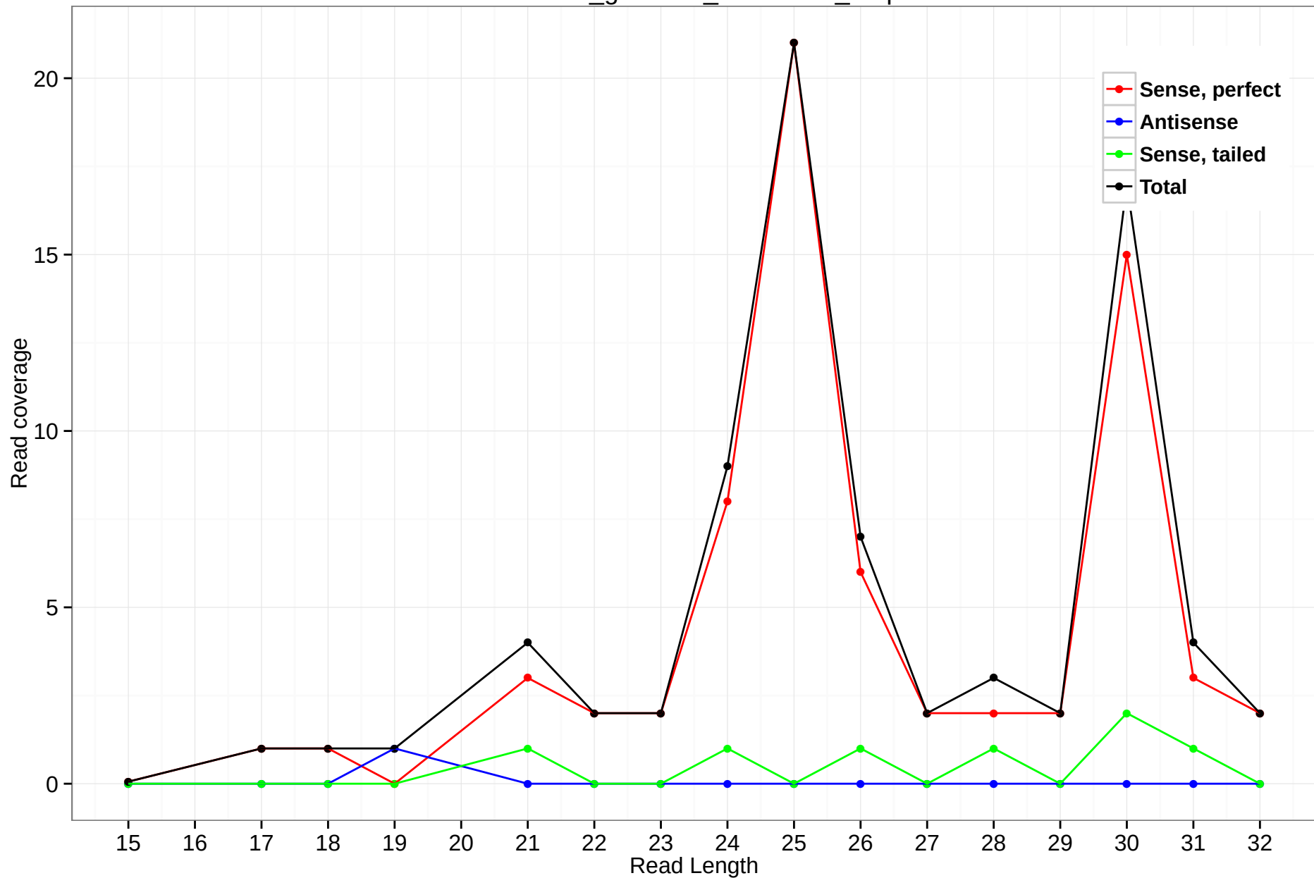
rheMac3_genscan_chr1.1107_5.3p
