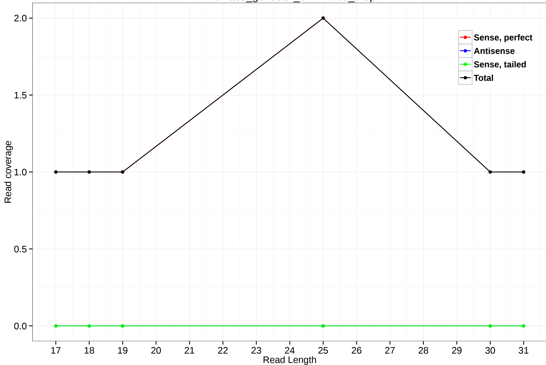
rheMac3_genscan_chr1.1055_9.5p
