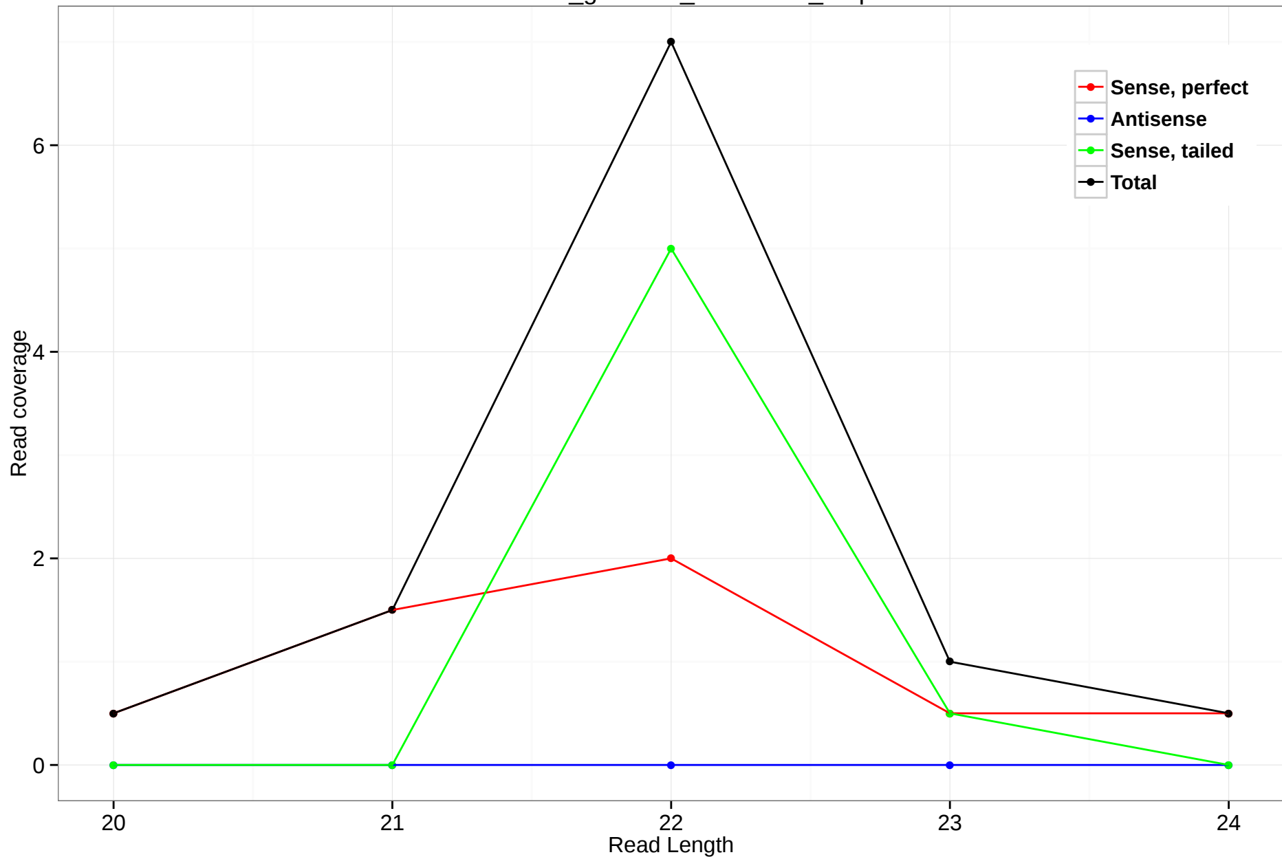
rheMac3_genscan_chr1.1015_8.3p
