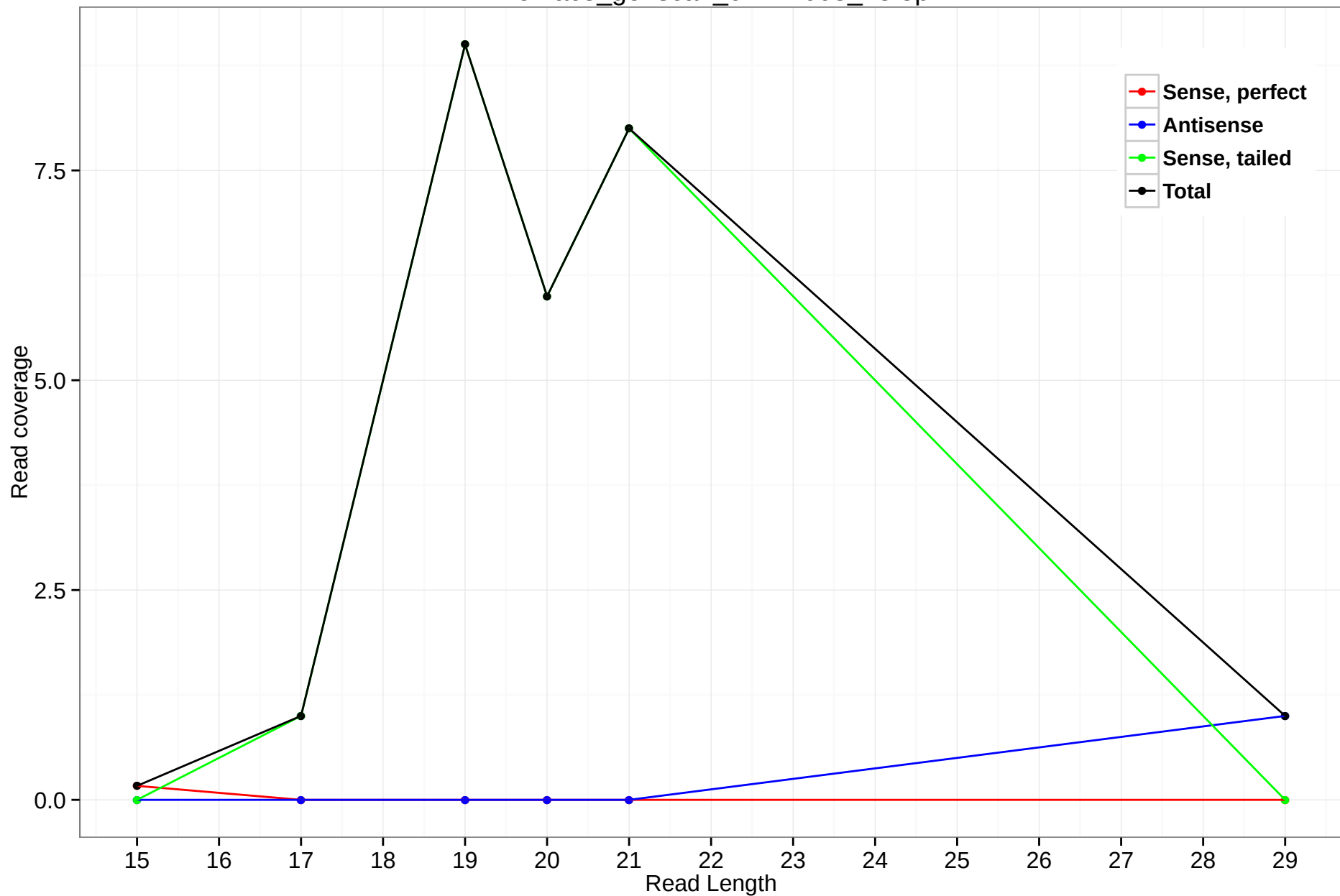
rheMac3_genscan_chr1.1003_28.5p
