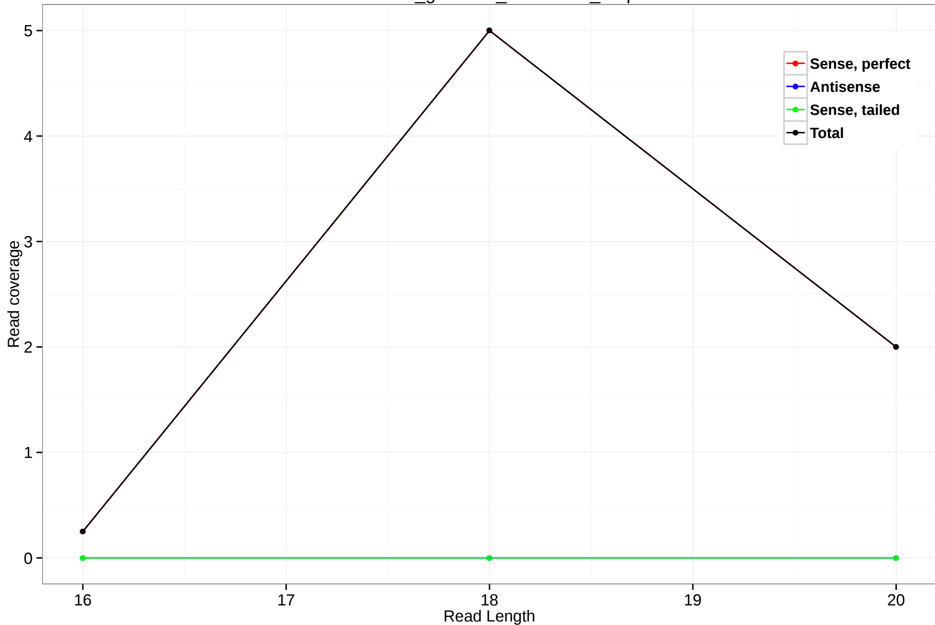
rheMac3_genscan_chr1.1003_0.5p
