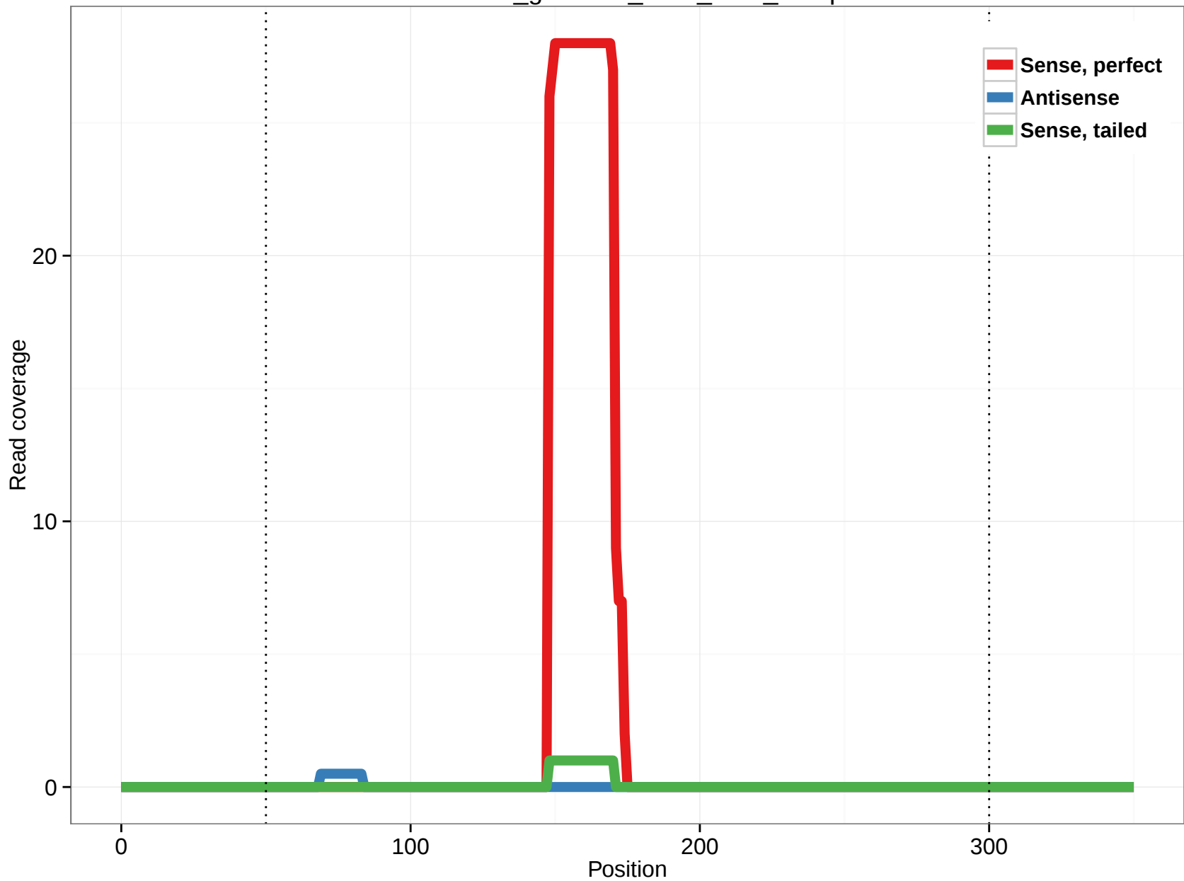
rheMac3_genscan_chrX_61.8_66.3p
