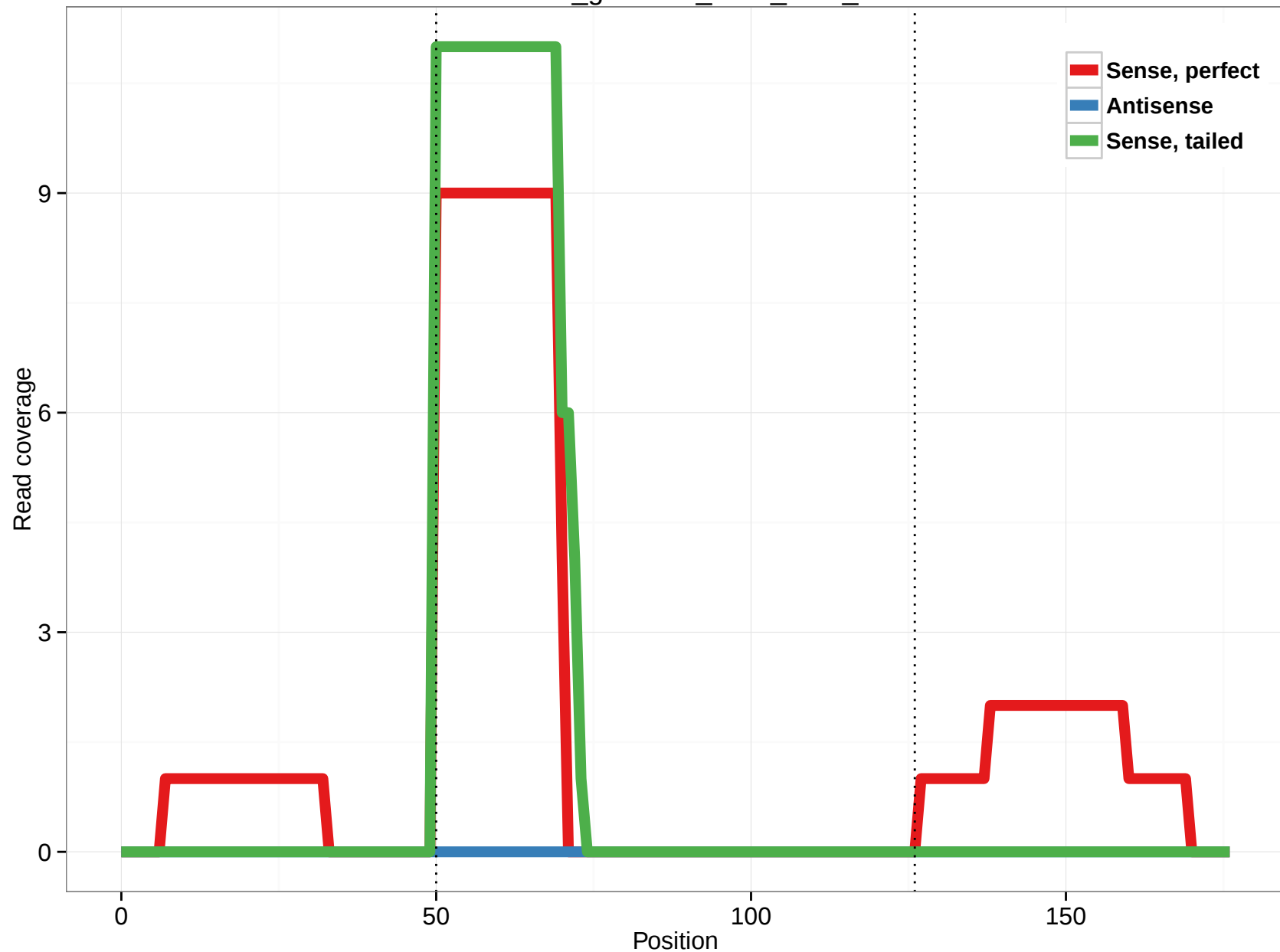
rheMac3_genscan_chrX_61.8_57
