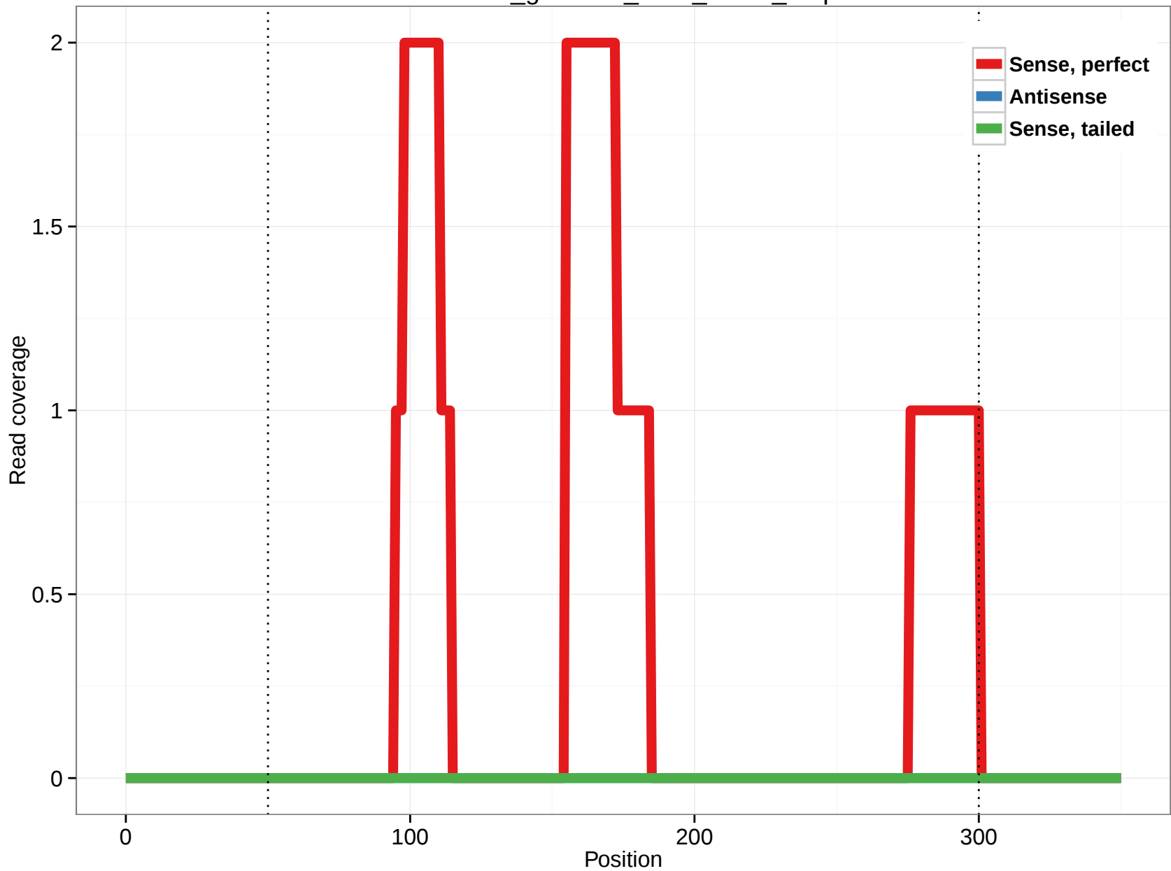
rheMac3_genscan_chrX_61.10_1.5p
