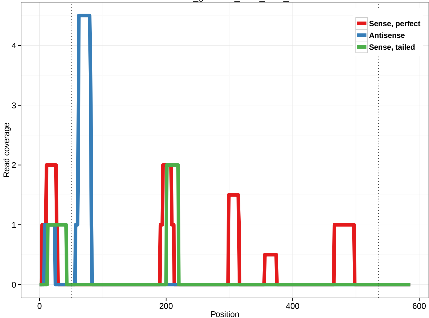
rheMac3_genscan_chrX_41.5_5
