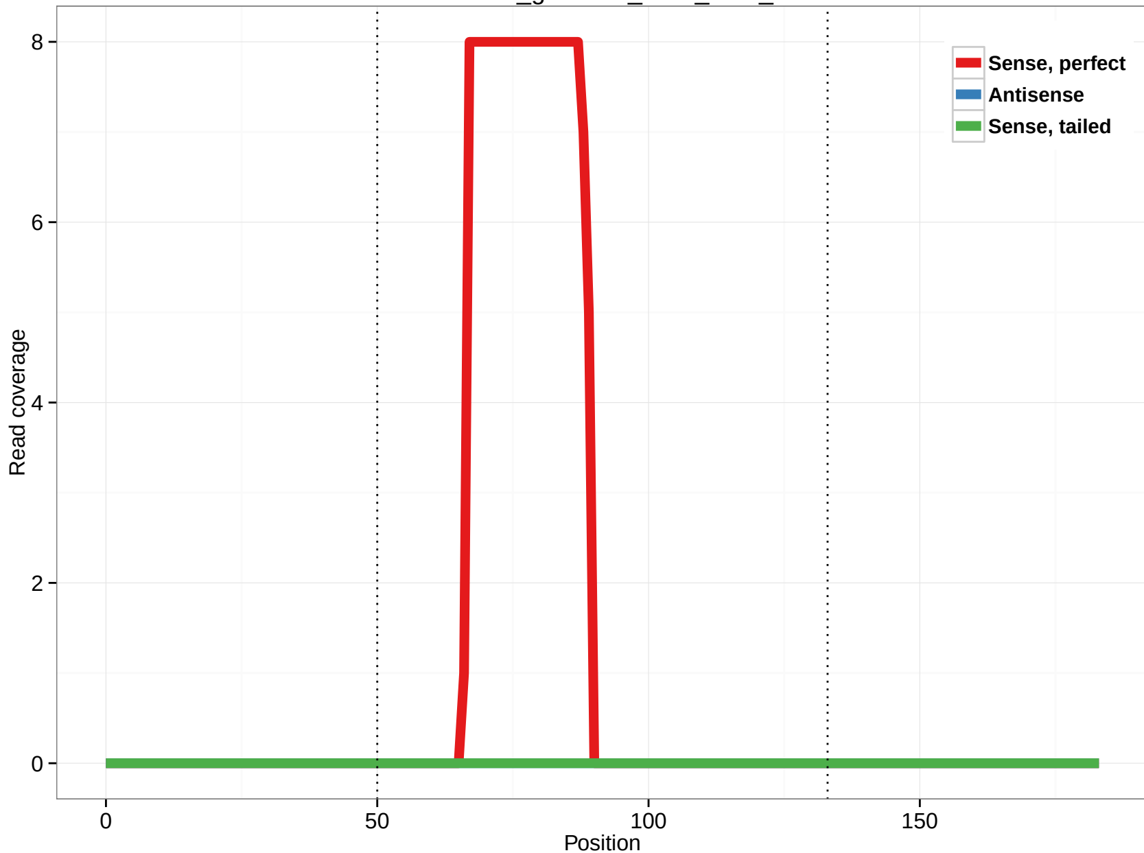
rheMac3_genscan_chrX_40.9_4
