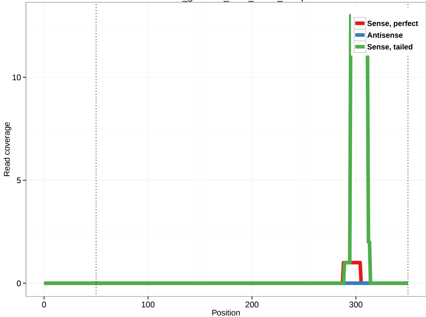
rheMac3_genscan_chrX_40.12_11.5p
