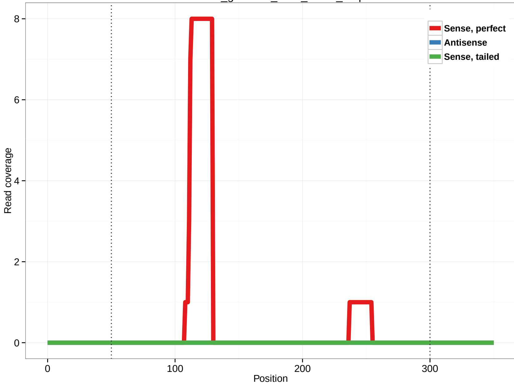
rheMac3_genscan_chrX_39.26_1.3p
