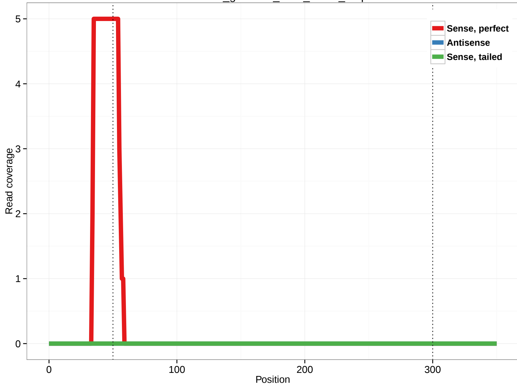
rheMac3_genscan_chrX_39.25_5.5p
