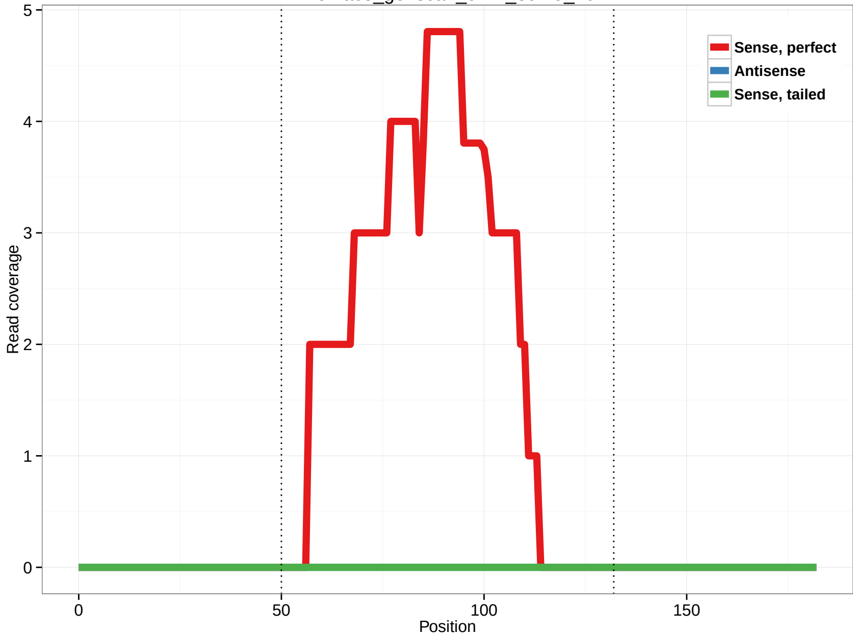
rheMac3_genscan_chrX_39.19_10
