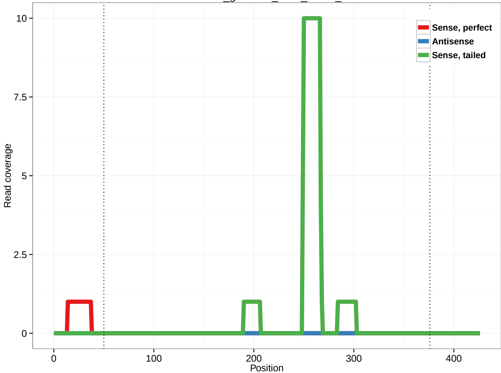
rheMac3_genscan_chrX_39.18_12
