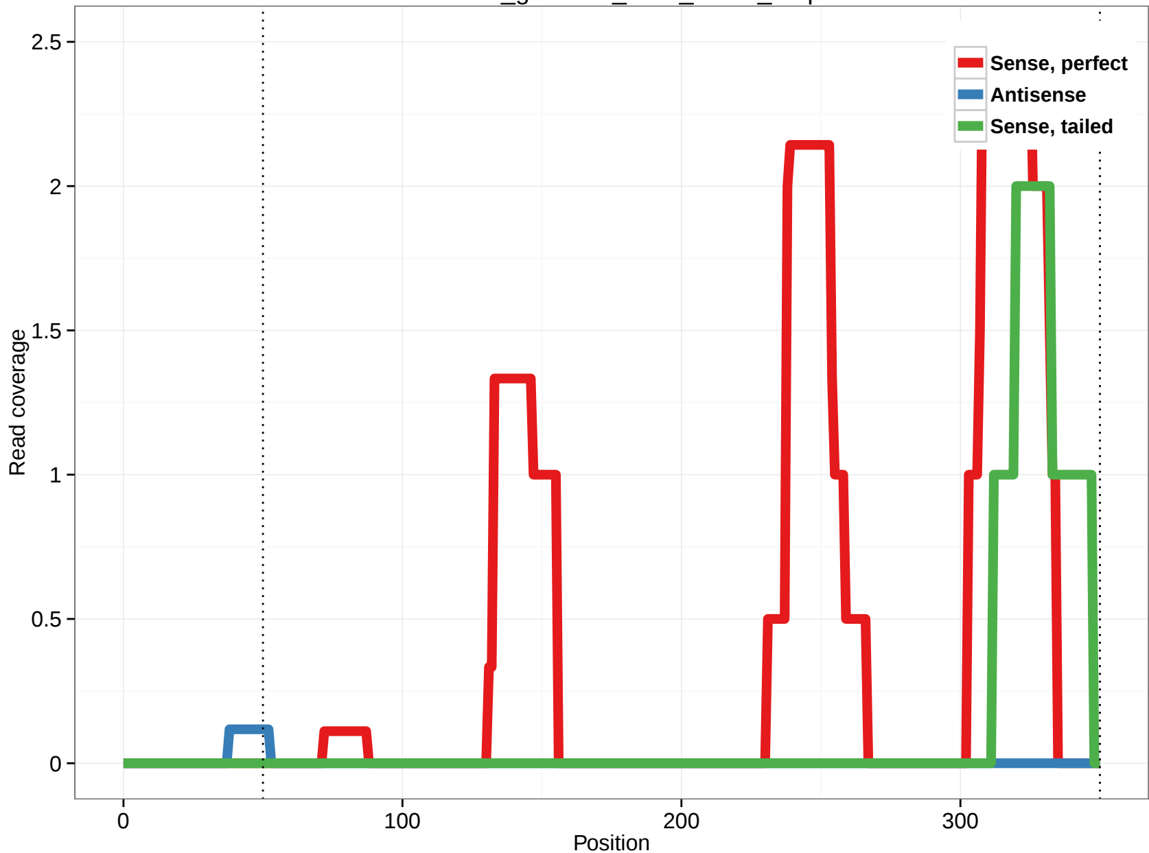
rheMac3_genscan_chrX_34.21_0.5p
