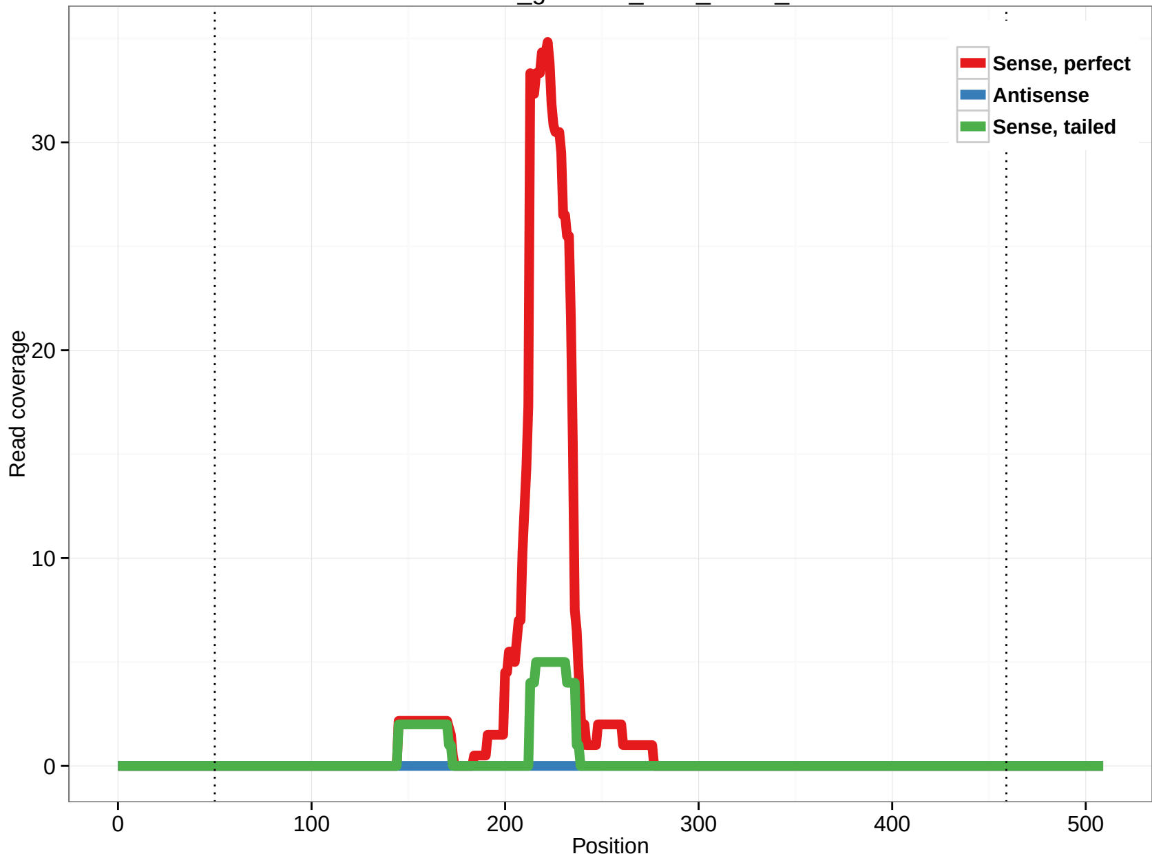
rheMac3_genscan_chrX_322.3_8
