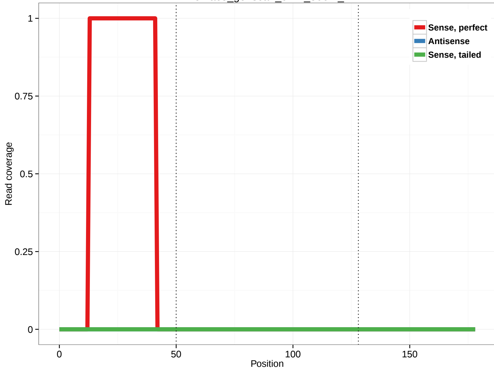
rheMac3_genscan_chrX_306.2_4
