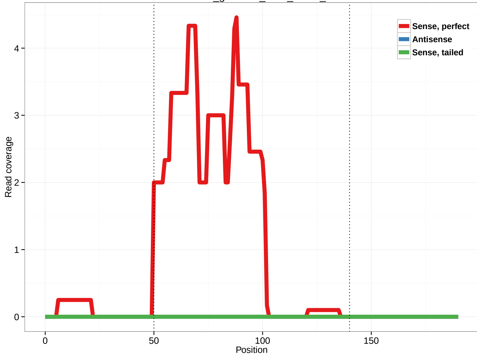
rheMac3_genscan_chrX_305.1_5
