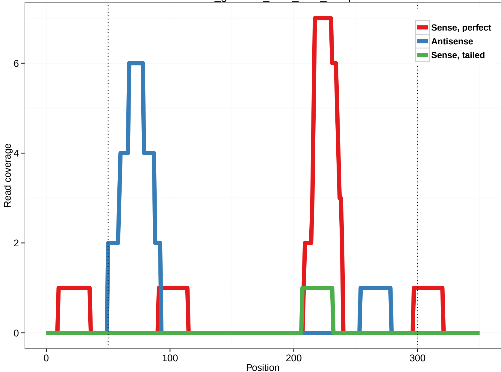
rheMac3_genscan_chrX_30.5_19.3p
