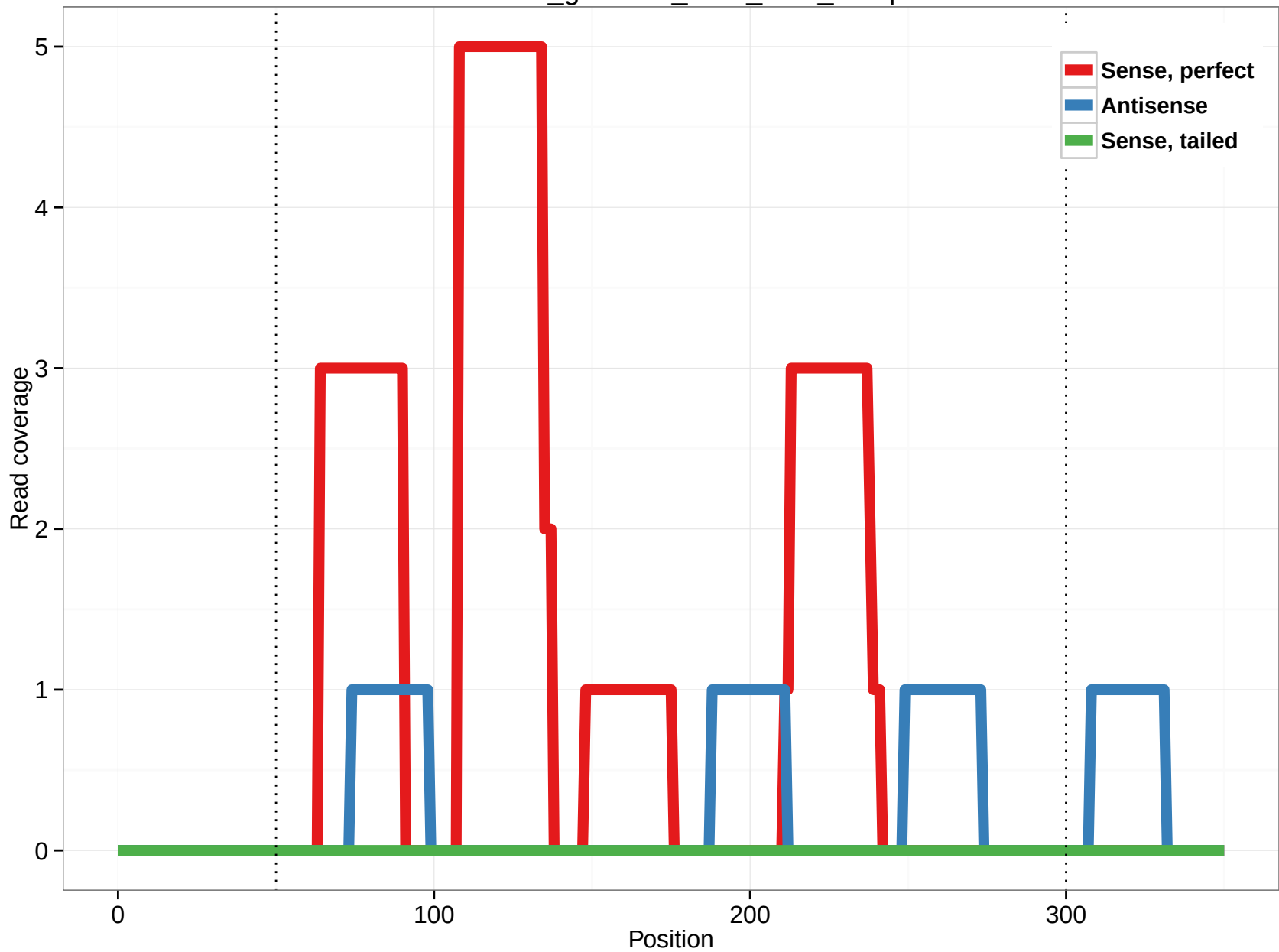
rheMac3_genscan_chrX_30.5_14.3p
