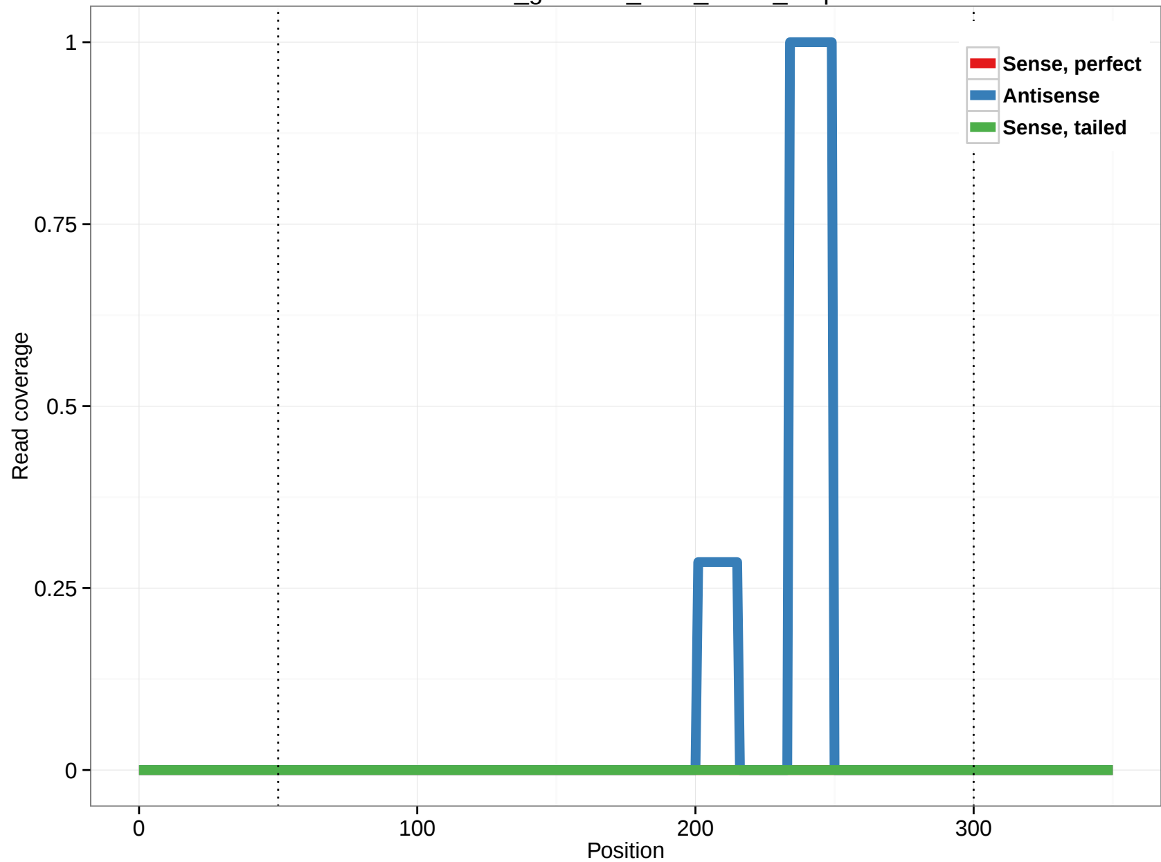
rheMac3_genscan_chrX_298.9_5.3p
