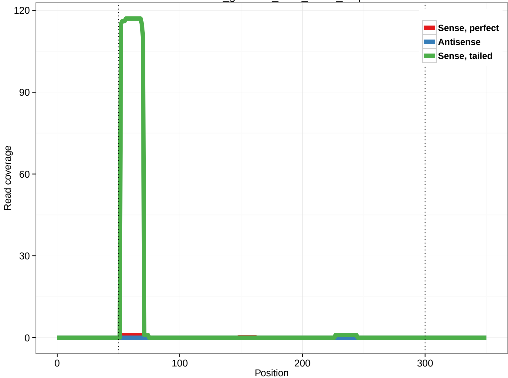
rheMac3_genscan_chrX_294.5_5.5p
