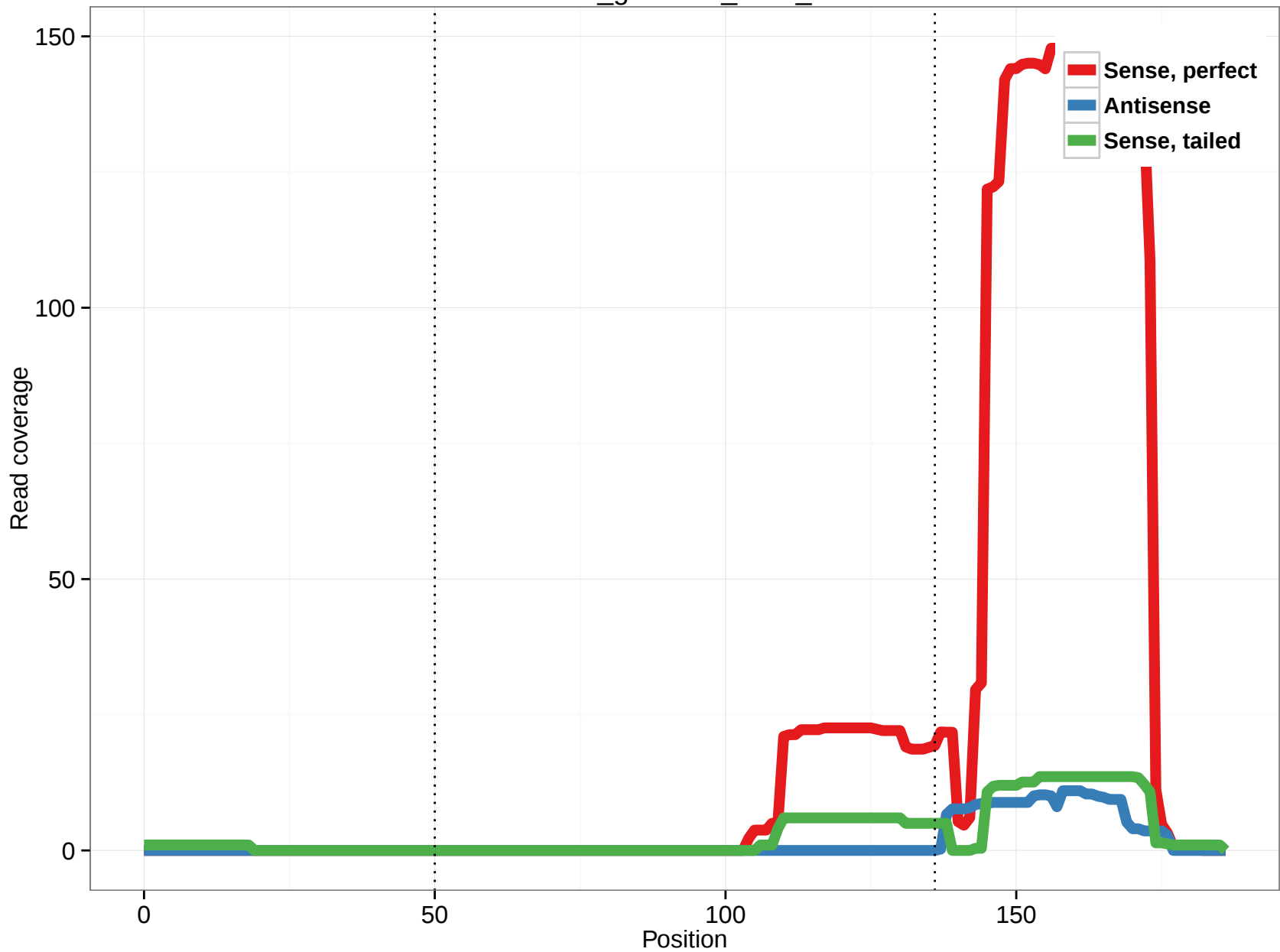
rheMac3_genscan_chrX_29.29
