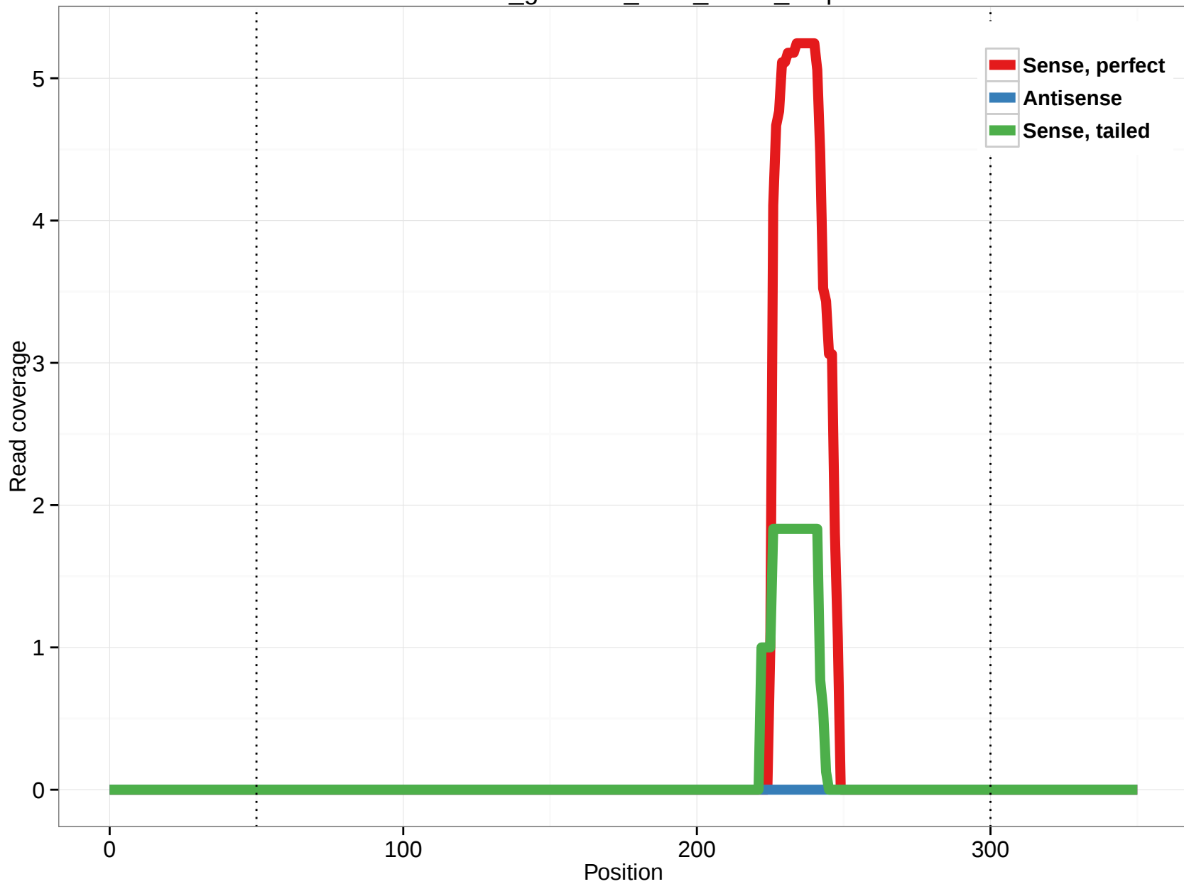
rheMac3_genscan_chrX_253.6_1.5p
