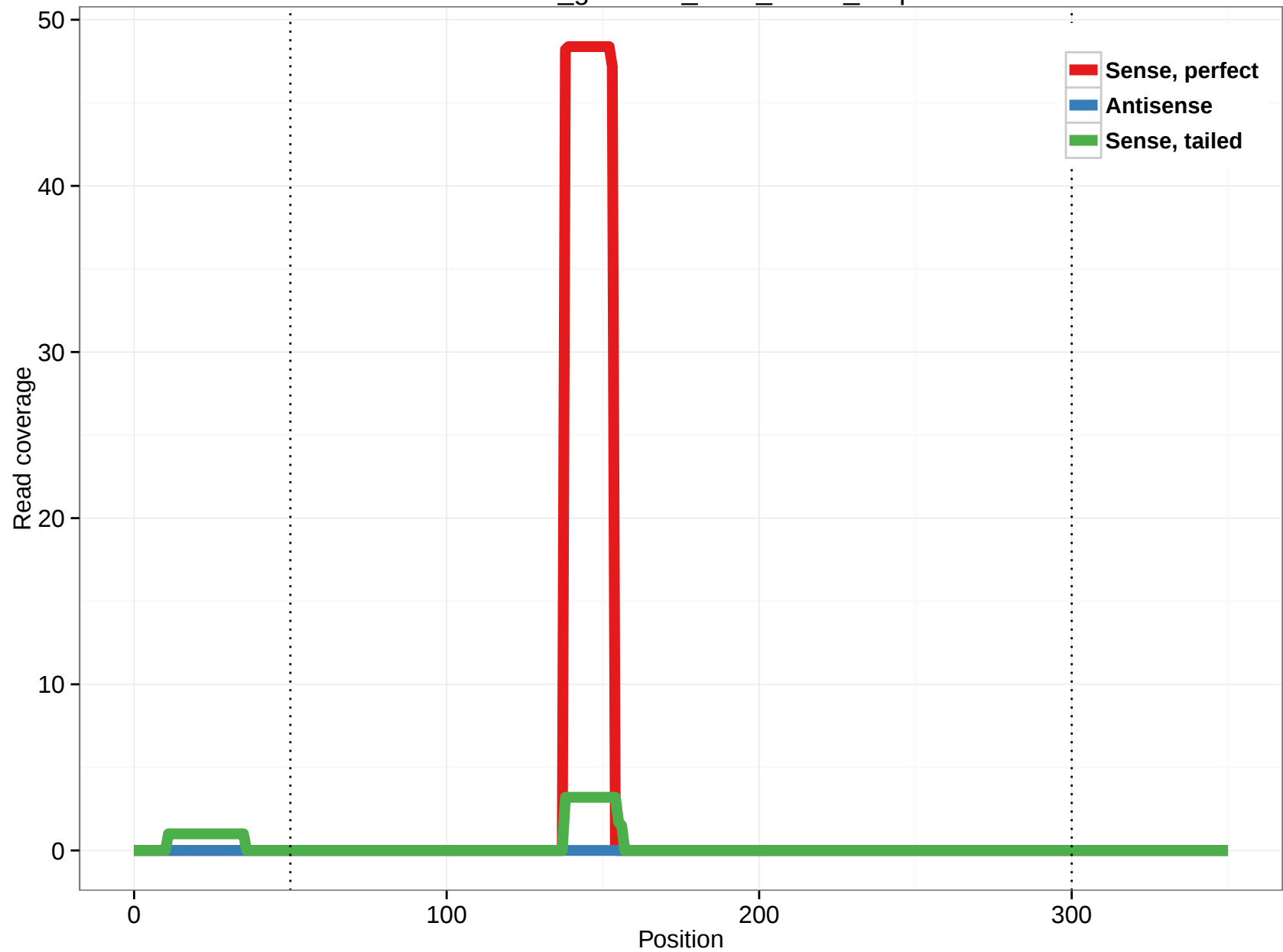
rheMac3_genscan_chrX_237.4_7.5p
