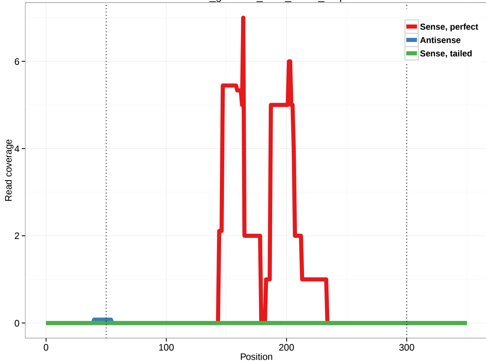
rheMac3_genscan_chrX_236.1_0.3p
