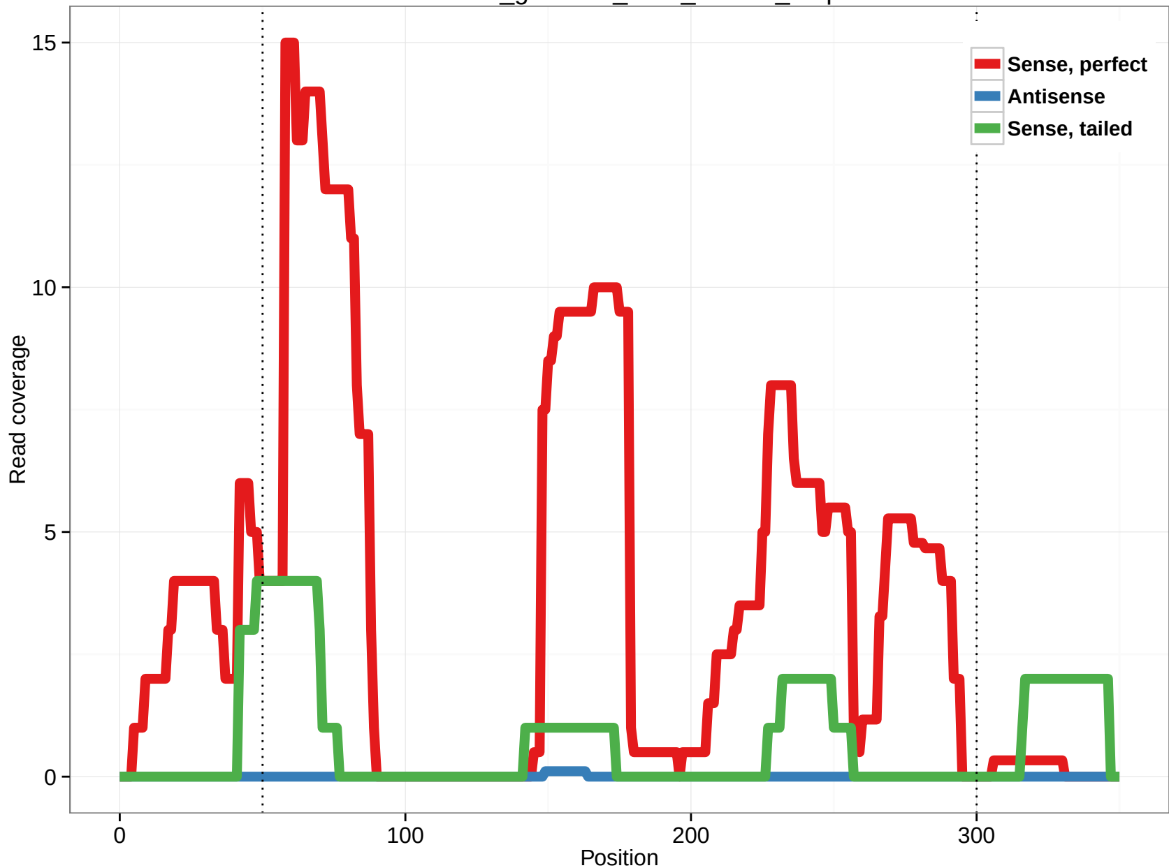
rheMac3_genscan_chrx_235.12_5.5p
